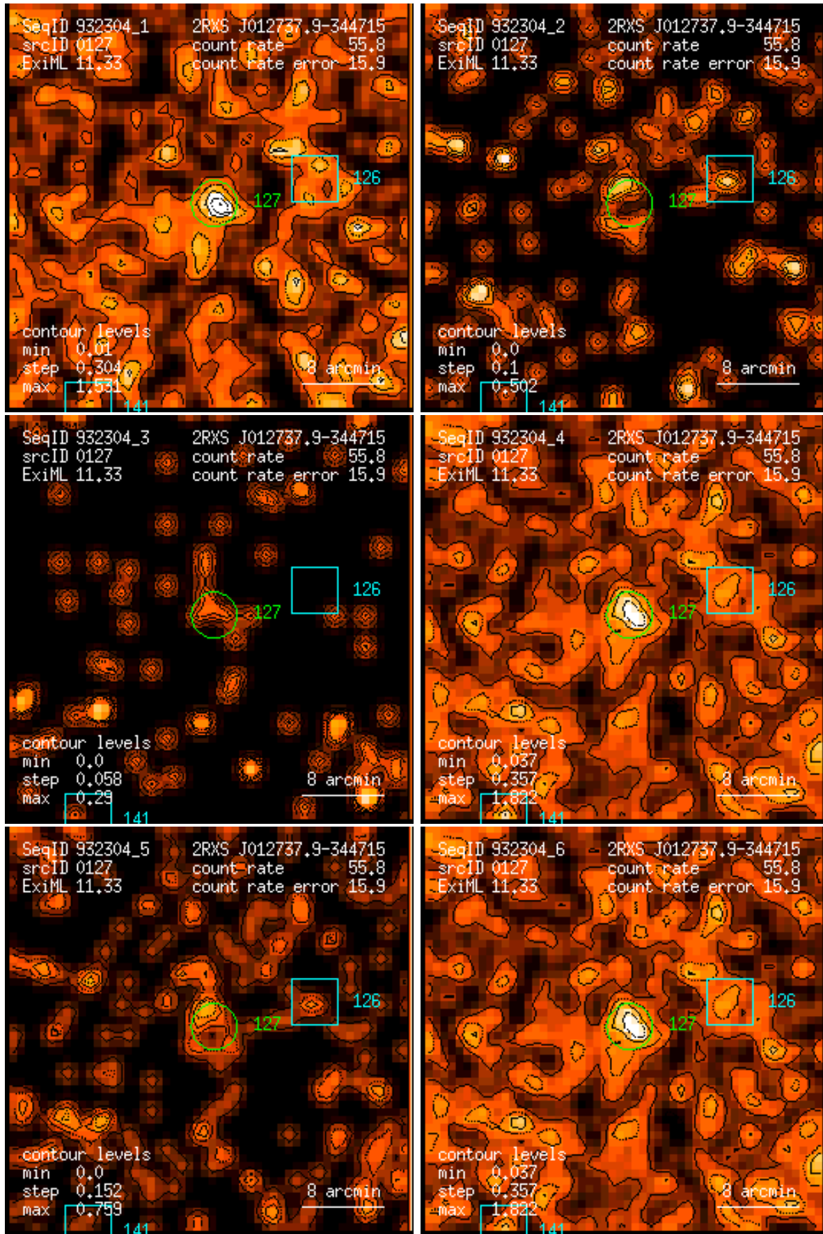
Figure 127: RASS 932304: detection 0127: band rate images, Gaussian filter: (1) PSPC channels 11 – 41, (2) 52 – 90, (3) 91 – 201, (4) 11 – 235, (5) 52 – 201, (6) 11 – 201. Broad band rates in counts/ks. Band rate contour levels in counts/ks/arcmin 2 .
