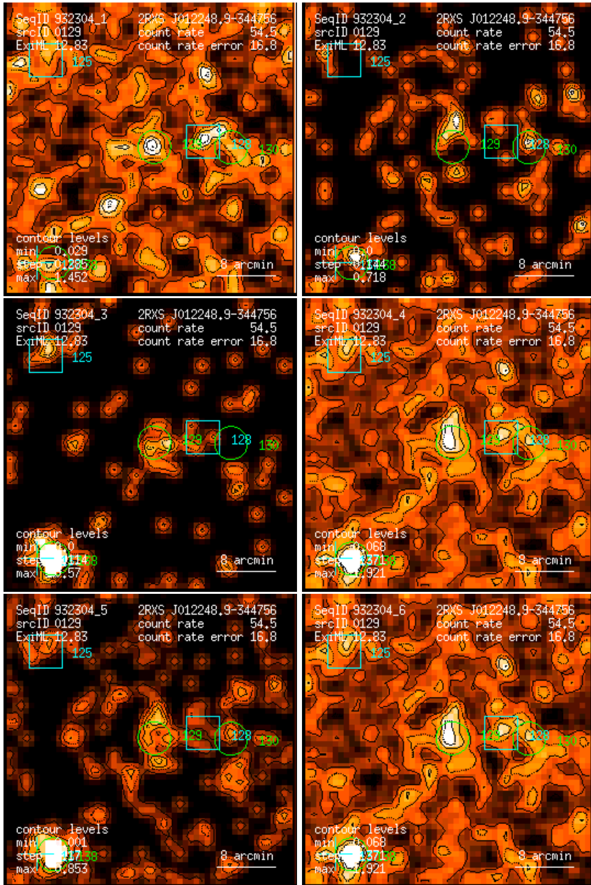
Figure 129: RASS 932304: detection 0129: band rate images, Gaussian filter: (1) PSPC channels 11 – 41, (2) 52 – 90, (3) 91 – 201, (4) 11 – 235, (5) 52 – 201, (6) 11 – 201. Broad band rates in counts/ks. Band rate contour levels in counts/ks/arcmin 2 .
