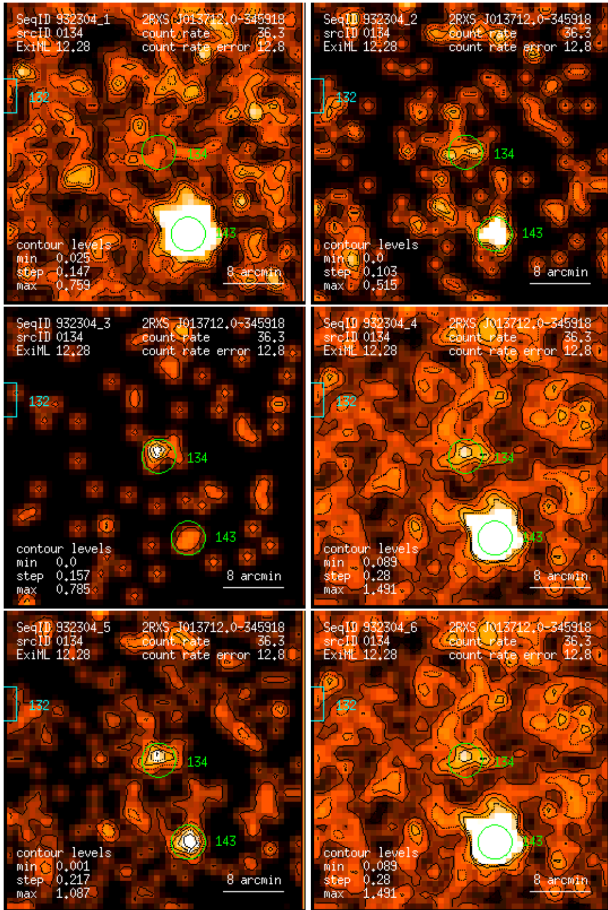
Figure 134: RASS 932304: detection 0134: band rate images, Gaussian filter: (1) PSPC channels 11 – 41, (2) 52 – 90, (3) 91 – 201, (4) 11 – 235, (5) 52 – 201, (6) 11 – 201. Broad band rates in counts/ks. Band rate contour levels in counts/ks/arcmin 2 .
