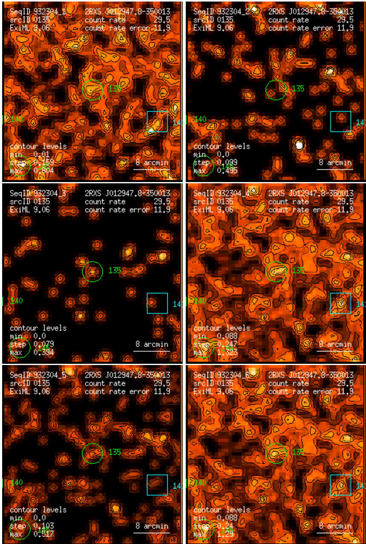
Figure 135: RASS 932304: detection 0135: band rate images, Gaussian filter: (1) PSPC channels 11 – 41, (2) 52 – 90, (3) 91 – 201, (4) 11 – 235, (5) 52 – 201, (6) 11 – 201. Broad band rates in counts/ks. Band rate contour levels in counts/ks/arcmin 2 .
