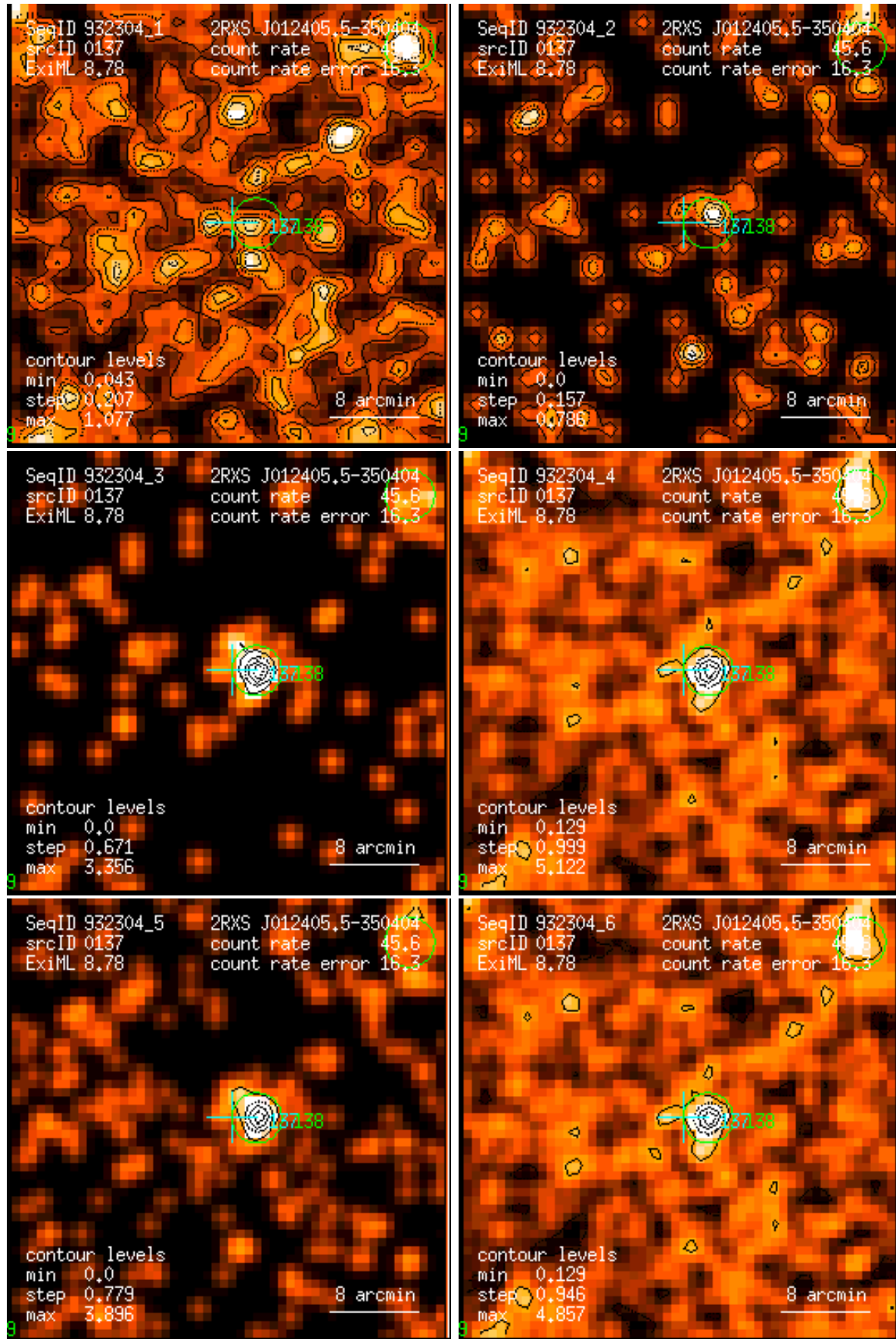
Figure 137: RASS 932304: detection 0137: band rate images, Gaussian filter: (1) PSPC channels 11 – 41, (2) 52 – 90, (3) 91 – 201, (4) 11 – 235, (5) 52 – 201, (6) 11 – 201. Broad band rates in counts/ks. Band rate contour levels in counts/ks/arcmin 2 .
