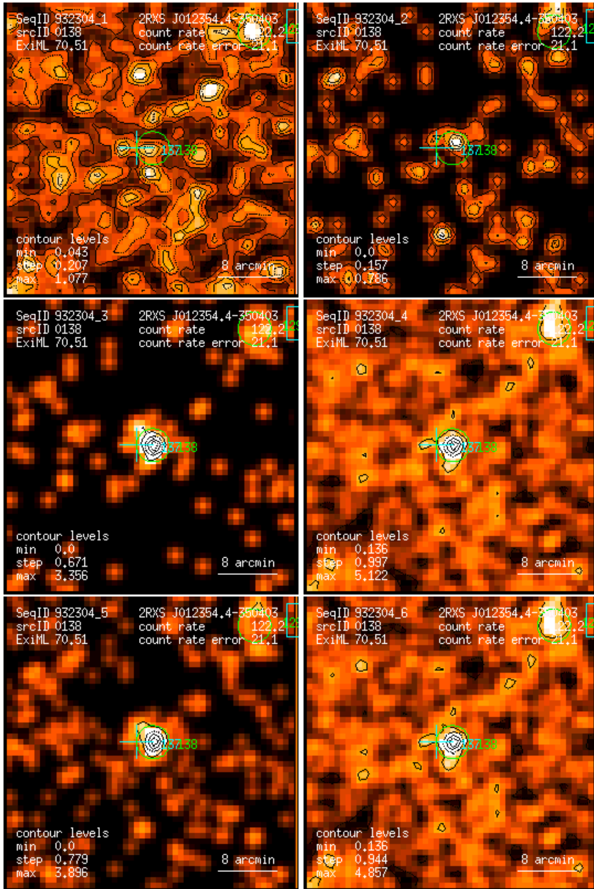
Figure 138: RASS 932304: detection 0138: band rate images, Gaussian filter: (1) PSPC channels 11 – 41, (2) 52 – 90, (3) 91 – 201, (4) 11 – 235, (5) 52 – 201, (6) 11 – 201. Broad band rates in counts/ks. Band rate contour levels in counts/ks/arcmin 2 .
