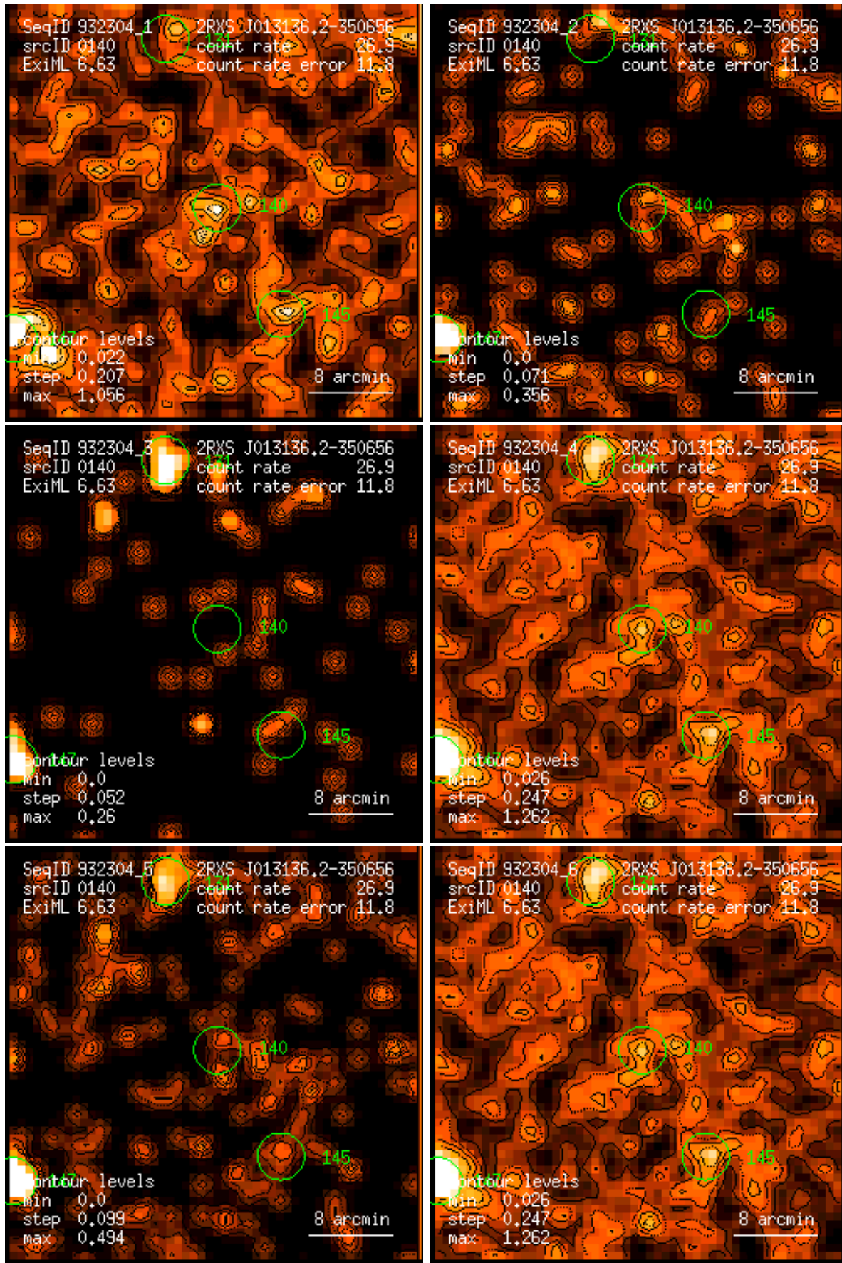
Figure 140: RASS 932304: detection 0140: band rate images, Gaussian filter: (1) PSPC channels 11 – 41, (2) 52 – 90, (3) 91 – 201, (4) 11 – 235, (5) 52 – 201, (6) 11 – 201. Broad band rates in counts/ks. Band rate contour levels in counts/ks/arcmin 2 .
