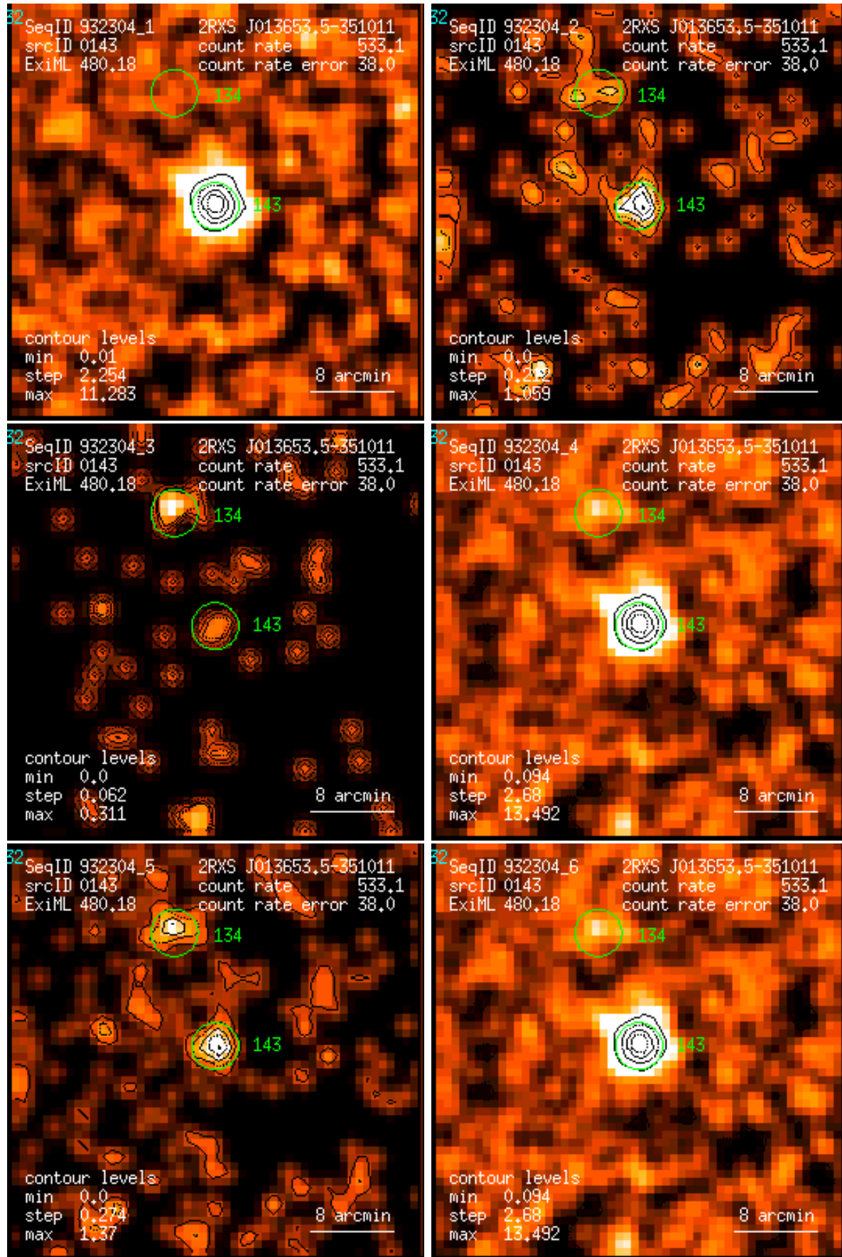
Figure 143: RASS 932304: detection 0143: band rate images, Gaussian filter: (1) PSPC channels 11 – 41, (2) 52 – 90, (3) 91 – 201, (4) 11 – 235, (5) 52 – 201, (6) 11 – 201. Broad band rates in counts/ks. Band rate contour levels in counts/ks/arcmin 2 .
