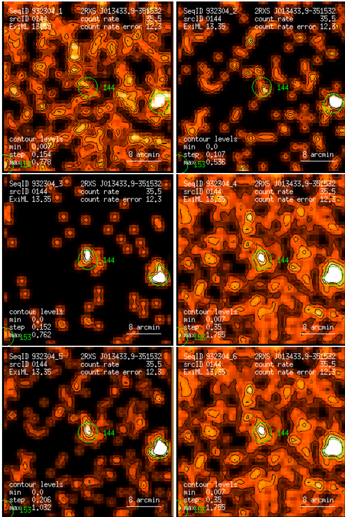
Figure 144: RASS 932304: detection 0144: band rate images, Gaussian filter: (1) PSPC channels 11 – 41, (2) 52 – 90, (3) 91 – 201, (4) 11 – 235, (5) 52 – 201, (6) 11 – 201. Broad band rates in counts/ks. Band rate contour levels in counts/ks/arcmin 2 .
