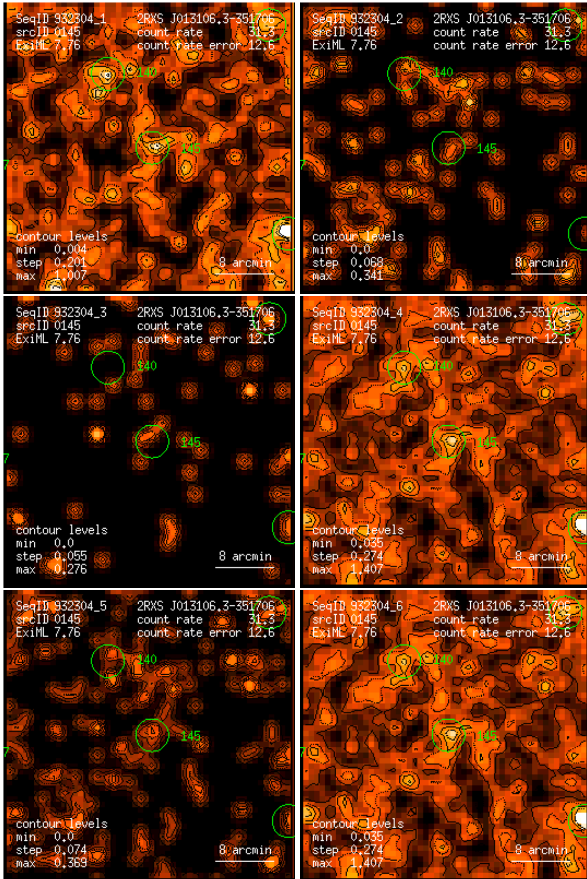
Figure 145: RASS 932304: detection 0145: band rate images, Gaussian filter: (1) PSPC channels 11 – 41, (2) 52 – 90, (3) 91 – 201, (4) 11 – 235, (5) 52 – 201, (6) 11 – 201. Broad band rates in counts/ks. Band rate contour levels in counts/ks/arcmin 2 .
