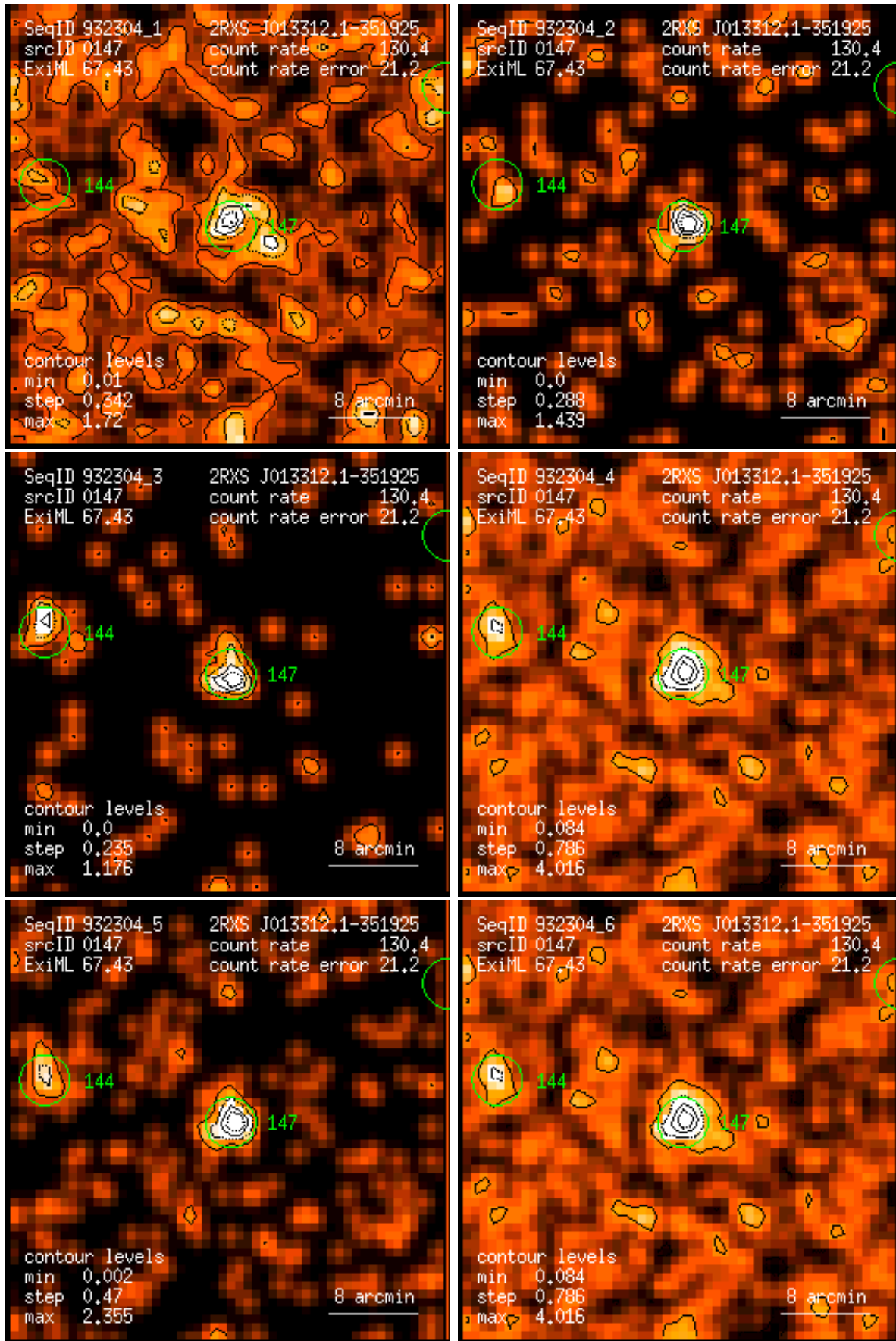
Figure 147: RASS 932304: detection 0147: band rate images, Gaussian filter: (1) PSPC channels 11 – 41, (2) 52 – 90, (3) 91 – 201, (4) 11 – 235, (5) 52 – 201, (6) 11 – 201. Broad band rates in counts/ks. Band rate contour levels in counts/ks/arcmin 2 .
