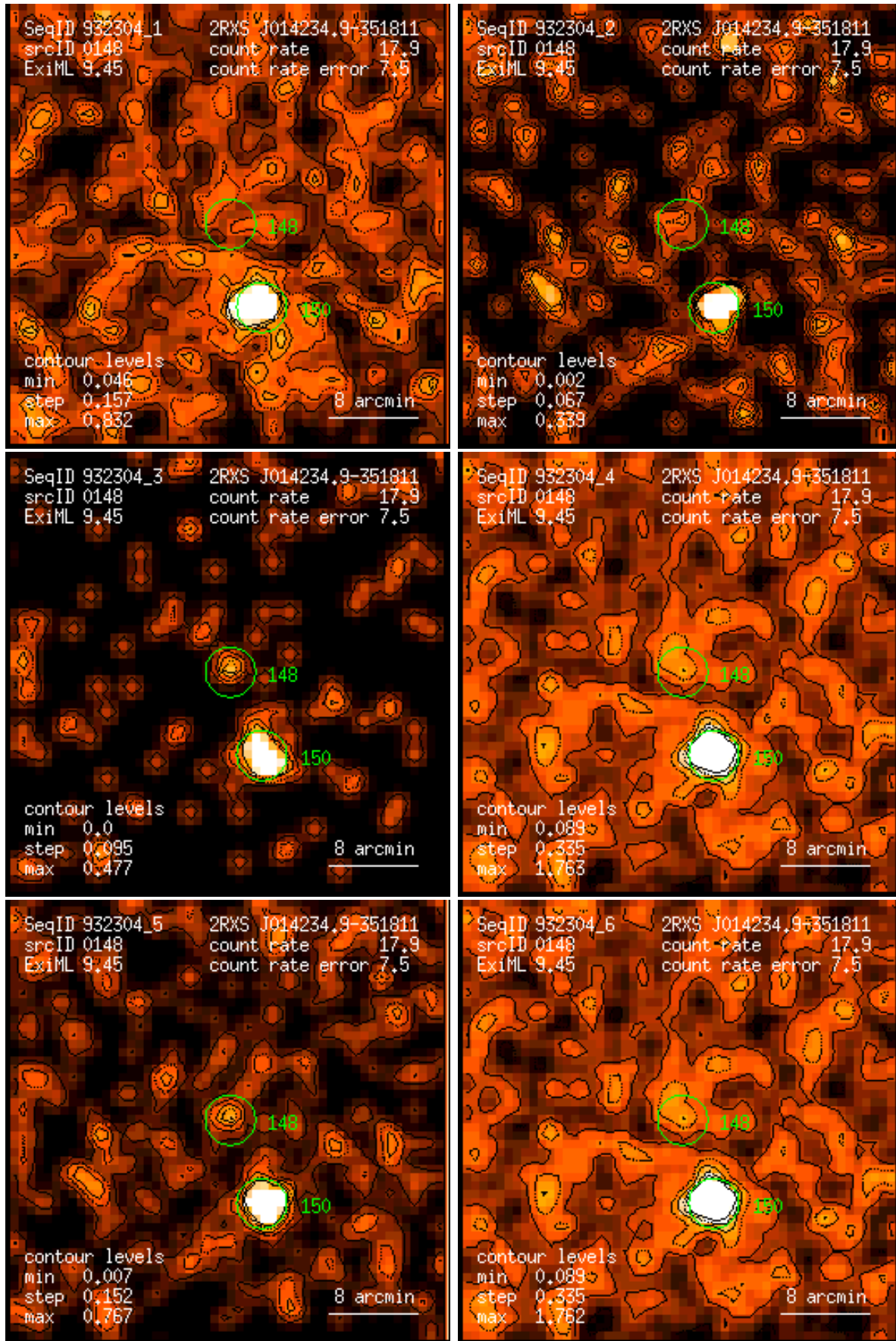
Figure 148: RASS 932304: detection 0148: band rate images, Gaussian filter: (1) PSPC channels 11 – 41, (2) 52 – 90, (3) 91 – 201, (4) 11 – 235, (5) 52 – 201, (6) 11 – 201. Broad band rates in counts/ks. Band rate contour levels in counts/ks/arcmin 2 .
