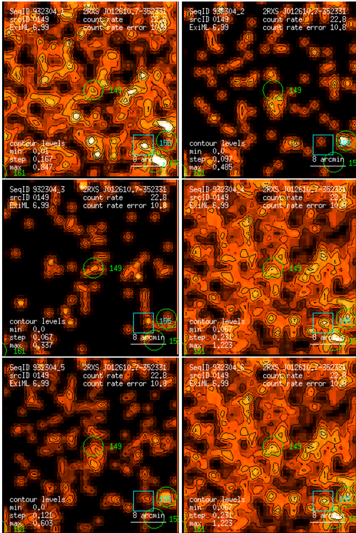
Figure 149: RASS 932304: detection 0149: band rate images, Gaussian filter: (1) PSPC channels 11 – 41, (2) 52 – 90, (3) 91 – 201, (4) 11 – 235, (5) 52 – 201, (6) 11 – 201. Broad band rates in counts/ks. Band rate contour levels in counts/ks/arcmin 2 .
