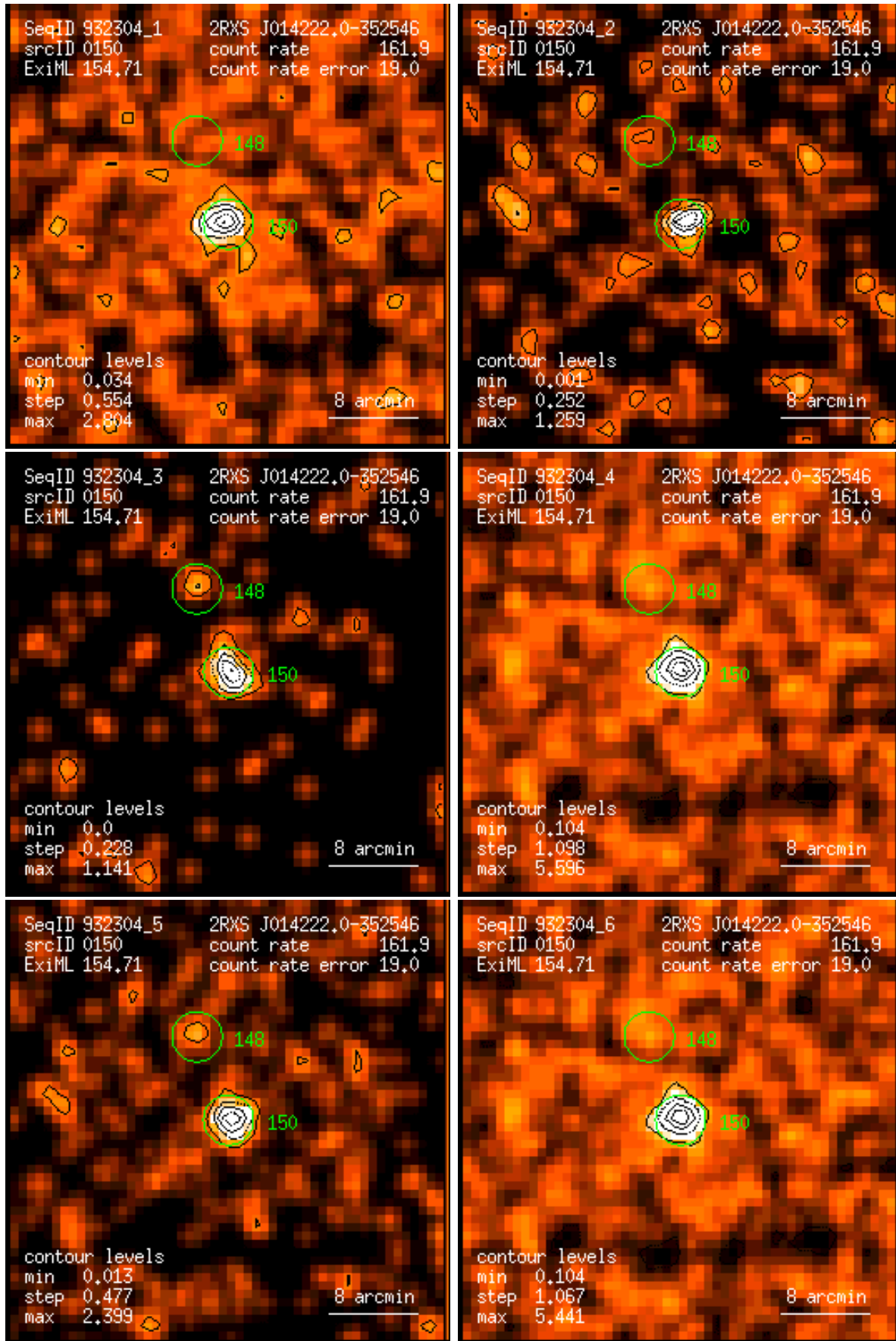
Figure 150: RASS 932304: detection 0150: band rate images, Gaussian filter: (1) PSPC channels 11 – 41, (2) 52 – 90, (3) 91 – 201, (4) 11 – 235, (5) 52 – 201, (6) 11 – 201. Broad band rates in counts/ks. Band rate contour levels in counts/ks/arcmin 2 .
