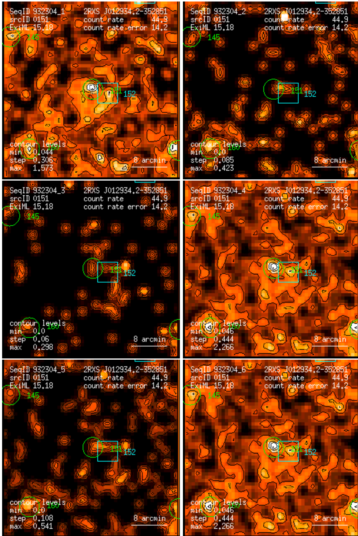
Figure 151: RASS 932304: detection 0151: band rate images, Gaussian filter: (1) PSPC channels 11 – 41, (2) 52 – 90, (3) 91 – 201, (4) 11 – 235, (5) 52 – 201, (6) 11 – 201. Broad band rates in counts/ks. Band rate contour levels in counts/ks/arcmin 2 .
