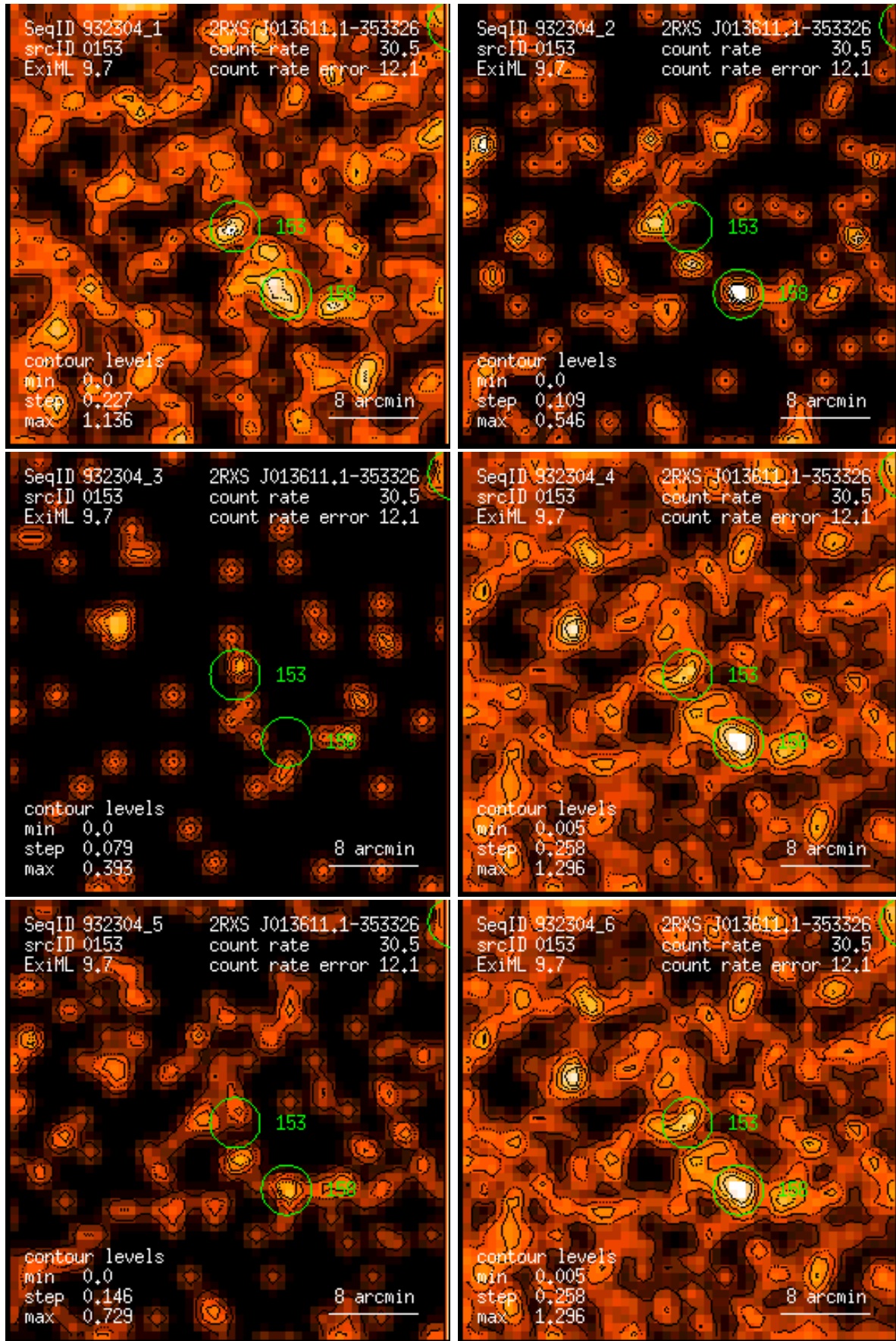
Figure 153: RASS 932304: detection 0153: band rate images, Gaussian filter: (1) PSPC channels 11 – 41, (2) 52 – 90, (3) 91 – 201, (4) 11 – 235, (5) 52 – 201, (6) 11 – 201. Broad band rates in counts/ks. Band rate contour levels in counts/ks/arcmin 2 .
