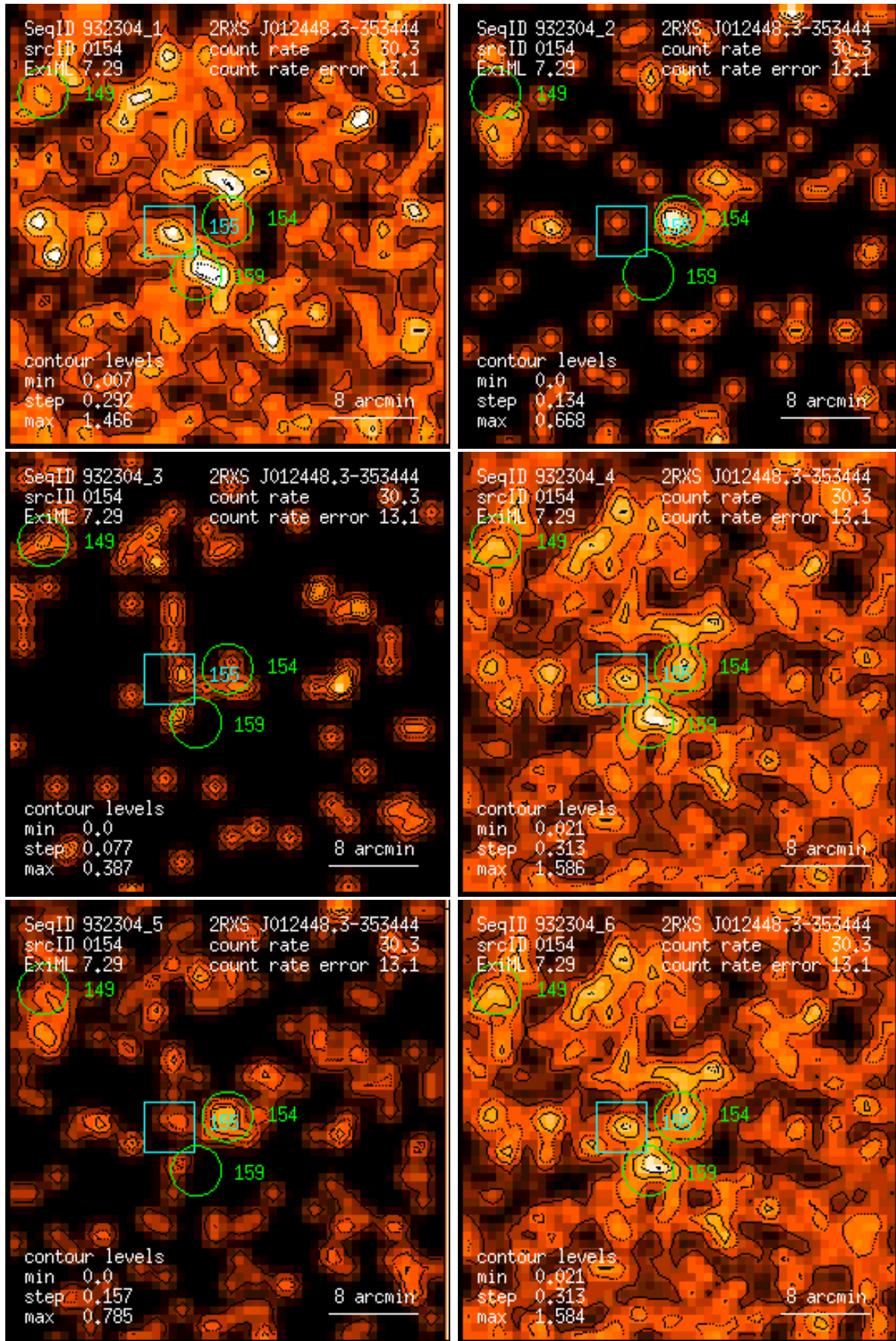
Figure 154: RASS 932304: detection 0154: band rate images, Gaussian filter: (1) PSPC channels 11 – 41, (2) 52 – 90, (3) 91 – 201, (4) 11 – 235, (5) 52 – 201, (6) 11 – 201. Broad band rates in counts/ks. Band rate contour levels in counts/ks/arcmin 2 .
