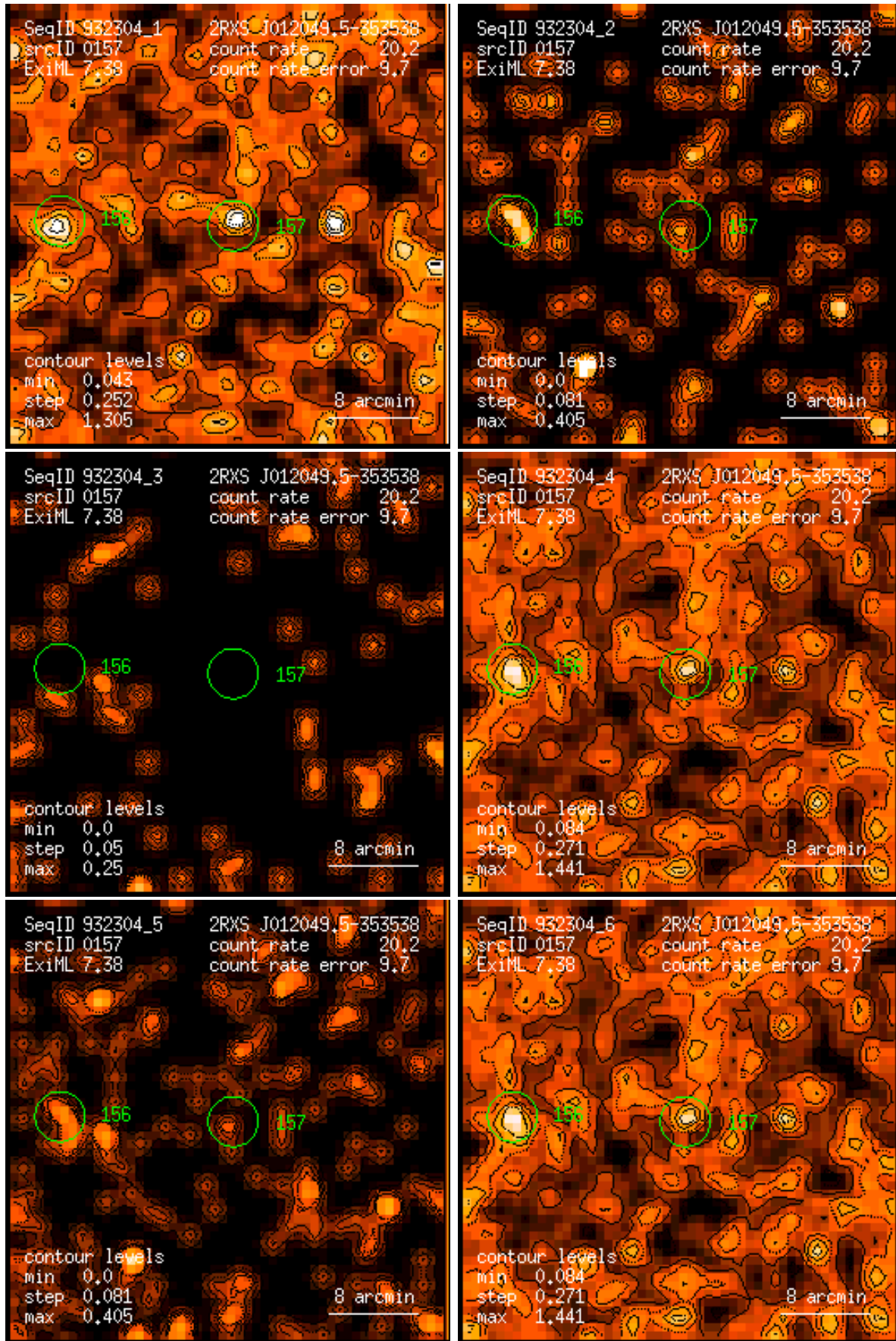
Figure 157: RASS 932304: detection 0157: band rate images, Gaussian filter: (1) PSPC channels 11 – 41, (2) 52 – 90, (3) 91 – 201, (4) 11 – 235, (5) 52 – 201, (6) 11 – 201. Broad band rates in counts/ks. Band rate contour levels in counts/ks/arcmin 2 .
