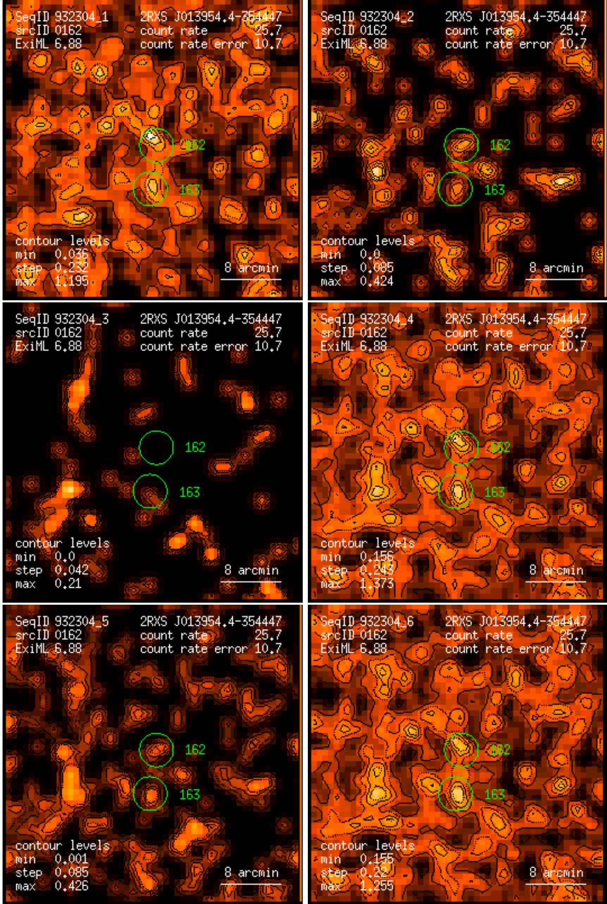
Figure 162: RASS 932304: detection 0162: band rate images, Gaussian filter: (1) PSPC channels 11 – 41, (2) 52 – 90, (3) 91 – 201, (4) 11 – 235, (5) 52 – 201, (6) 11 – 201. Broad band rates in counts/ks. Band rate contour levels in counts/ks/arcmin 2 .
