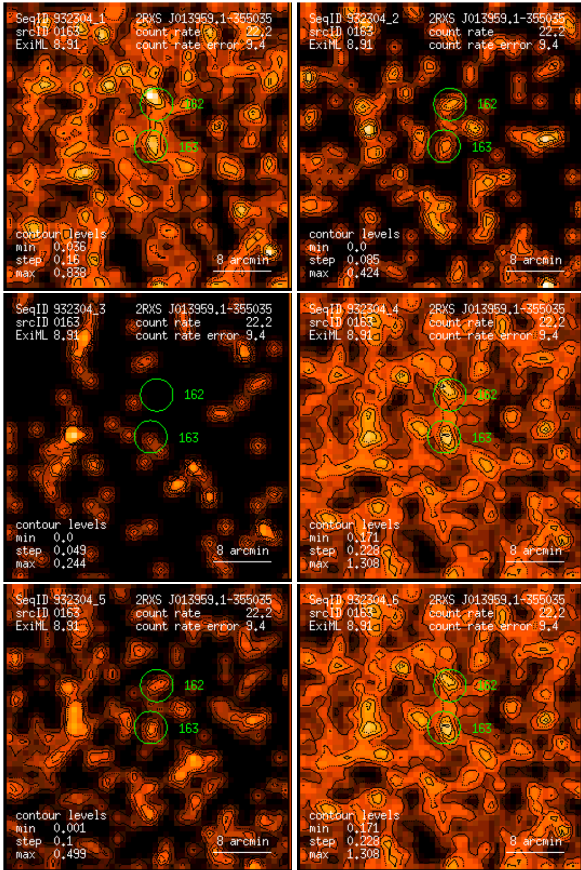
Figure 163: RASS 932304: detection 0163: band rate images, Gaussian filter: (1) PSPC channels 11 – 41, (2) 52 – 90, (3) 91 – 201, (4) 11 – 235, (5) 52 – 201, (6) 11 – 201. Broad band rates in counts/ks. Band rate contour levels in counts/ks/arcmin 2 .
