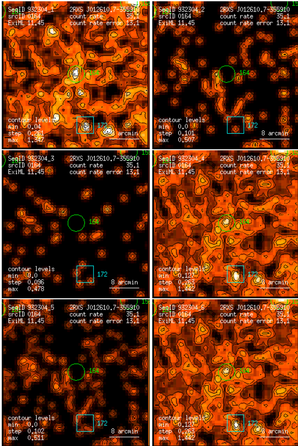
Figure 164: RASS 932304: detection 0164: band rate images, Gaussian filter: (1) PSPC channels 11 – 41, (2) 52 – 90, (3) 91 – 201, (4) 11 – 235, (5) 52 – 201, (6) 11 – 201. Broad band rates in counts/ks. Band rate contour levels in counts/ks/arcmin 2 .
