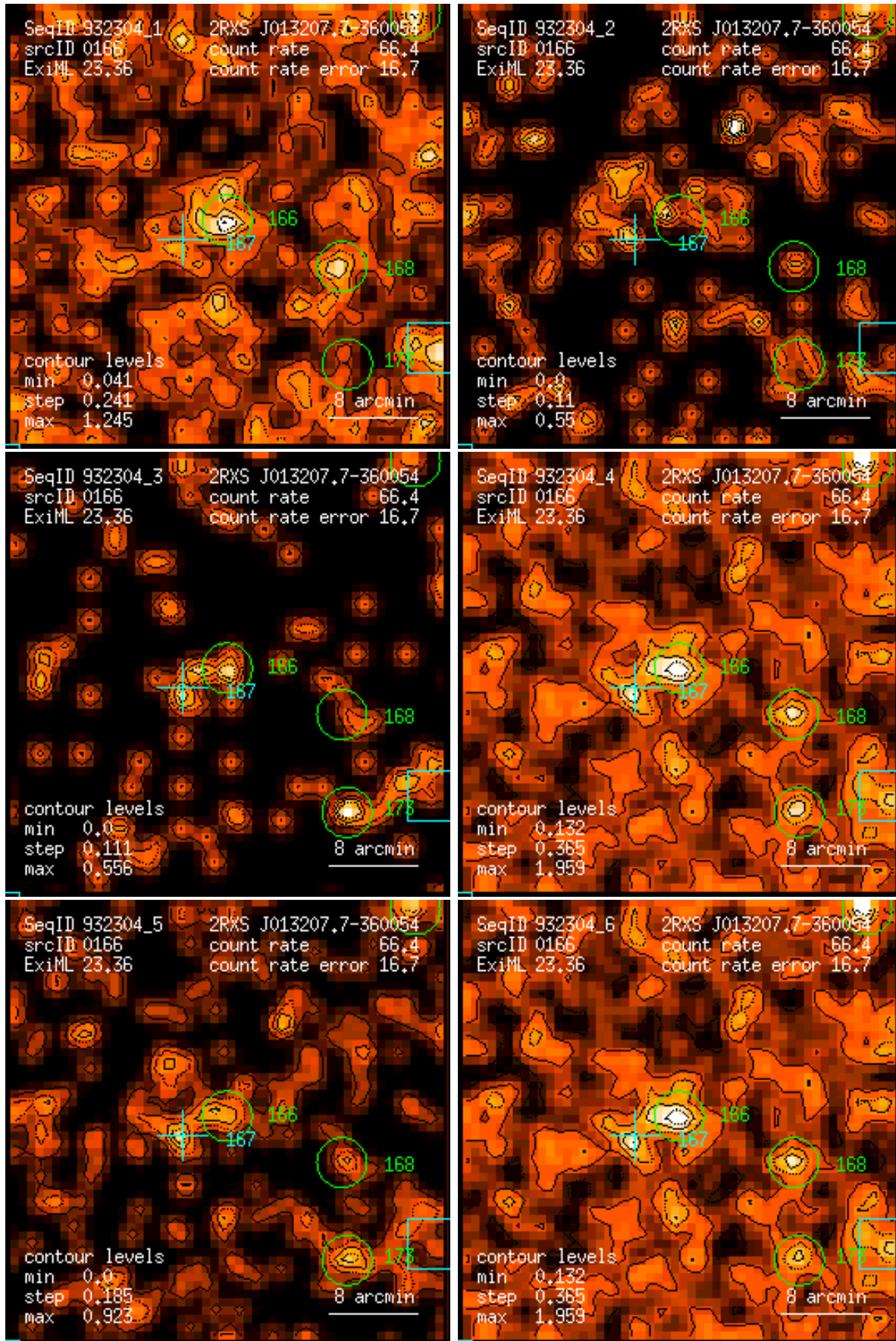
Figure 166: RASS 932304: detection 0166: band rate images, Gaussian filter: (1) PSPC channels 11 – 41, (2) 52 – 90, (3) 91 – 201, (4) 11 – 235, (5) 52 – 201, (6) 11 – 201. Broad band rates in counts/ks. Band rate contour levels in counts/ks/arcmin 2 .
