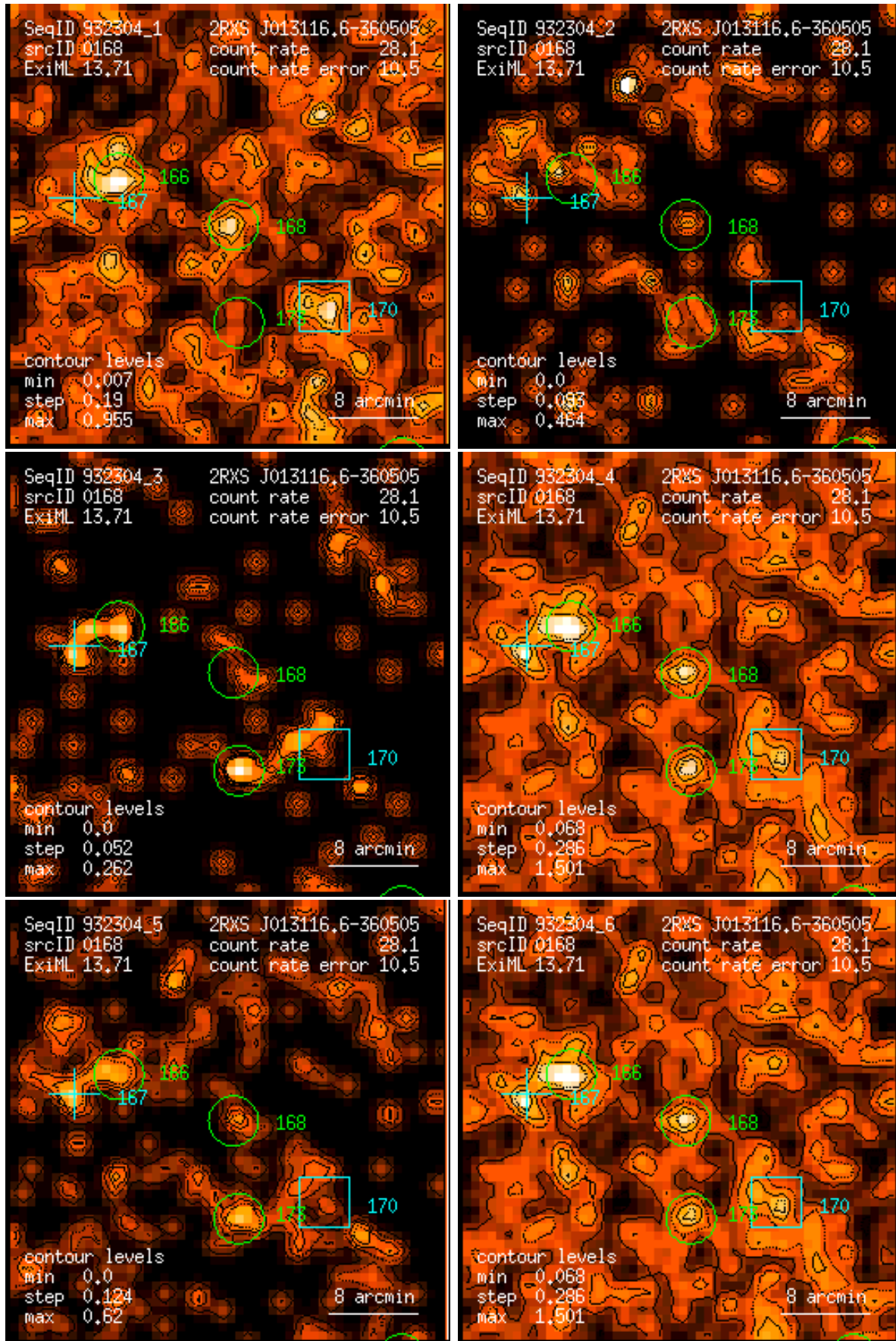
Figure 168: RASS 932304: detection 0168: band rate images, Gaussian filter: (1) PSPC channels 11 – 41, (2) 52 – 90, (3) 91 – 201, (4) 11 – 235, (5) 52 – 201, (6) 11 – 201. Broad band rates in counts/ks. Band rate contour levels in counts/ks/arcmin 2 .
