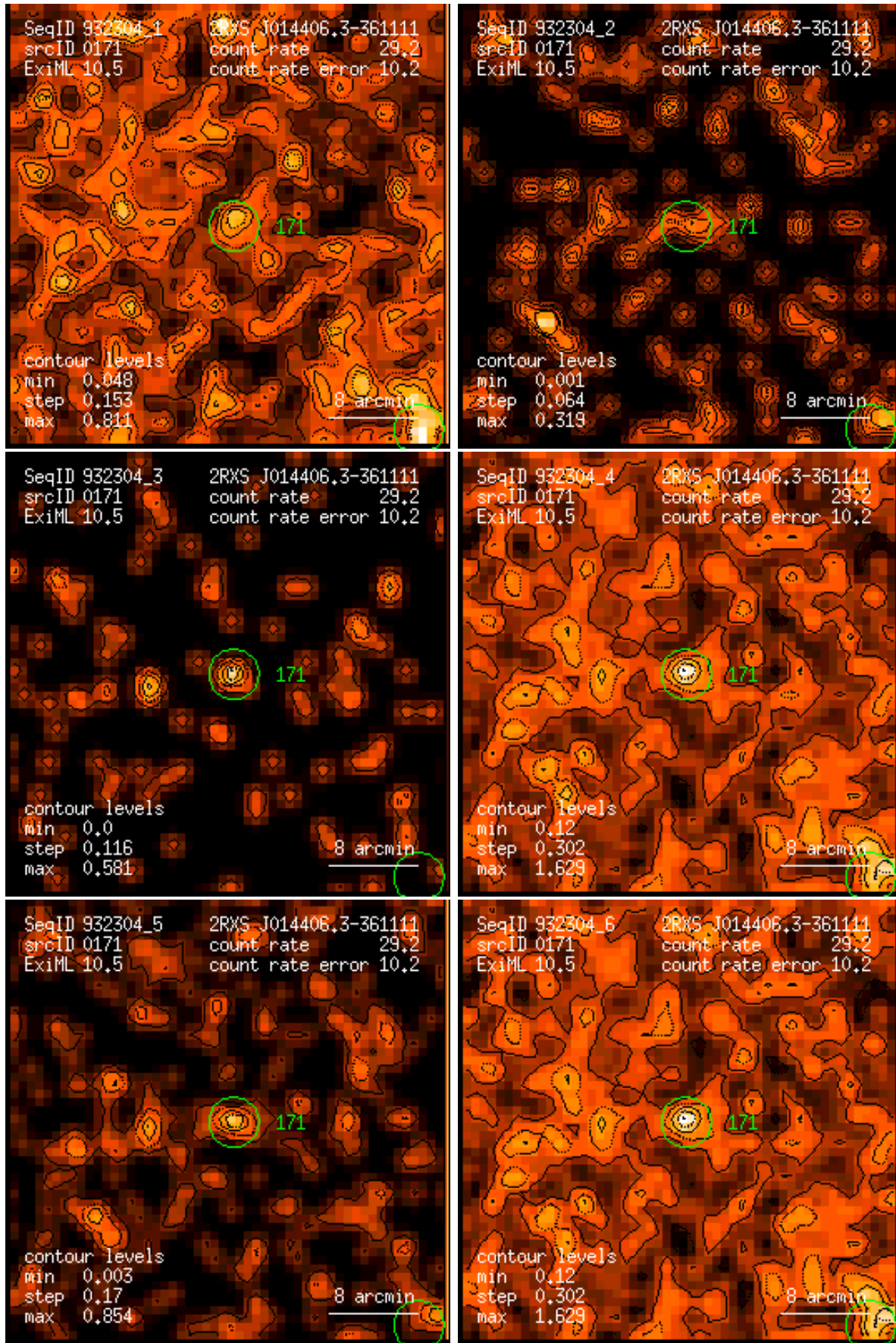
Figure 171: RASS 932304: detection 0171: band rate images, Gaussian filter: (1) PSPC channels 11 – 41, (2) 52 – 90, (3) 91 – 201, (4) 11 – 235, (5) 52 – 201, (6) 11 – 201. Broad band rates in counts/ks. Band rate contour levels in counts/ks/arcmin 2 .
