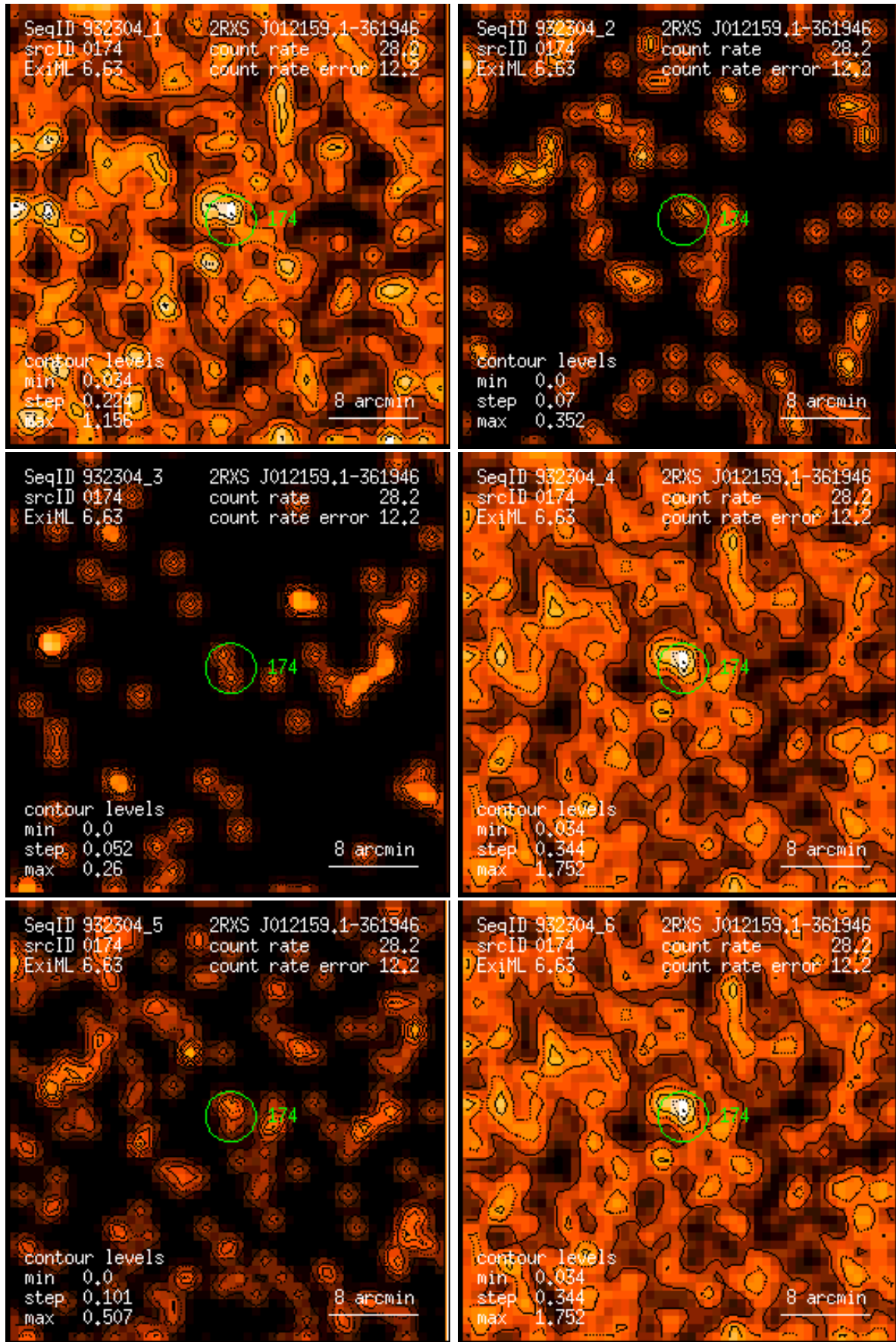
Figure 174: RASS 932304: detection 0174: band rate images, Gaussian filter: (1) PSPC channels 11 – 41, (2) 52 – 90, (3) 91 – 201, (4) 11 – 235, (5) 52 – 201, (6) 11 – 201. Broad band rates in counts/ks. Band rate contour levels in counts/ks/arcmin 2 .
