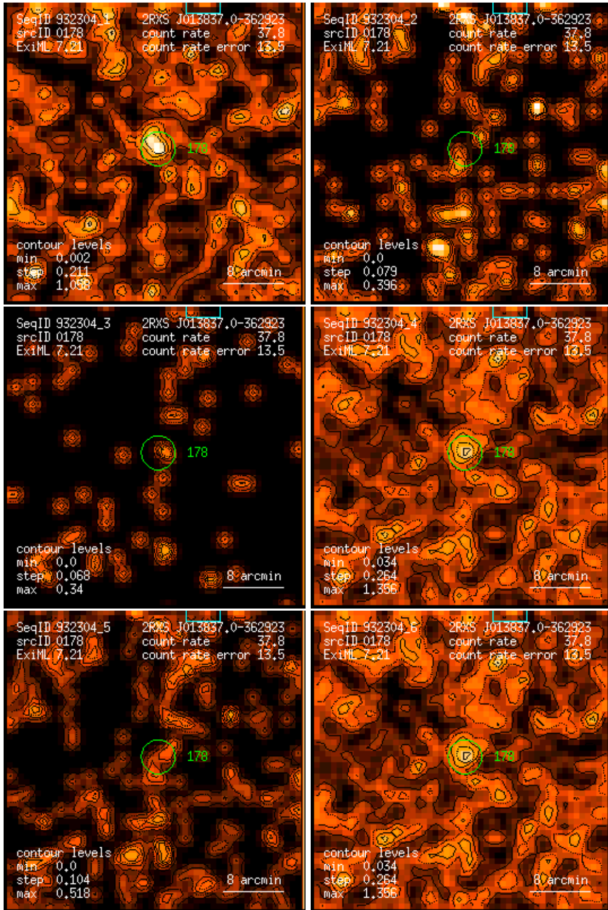
Figure 178: RASS 932304: detection 0178: band rate images, Gaussian filter: (1) PSPC channels 11 – 41, (2) 52 – 90, (3) 91 – 201, (4) 11 – 235, (5) 52 – 201, (6) 11 – 201. Broad band rates in counts/ks. Band rate contour levels in counts/ks/arcmin 2 .
