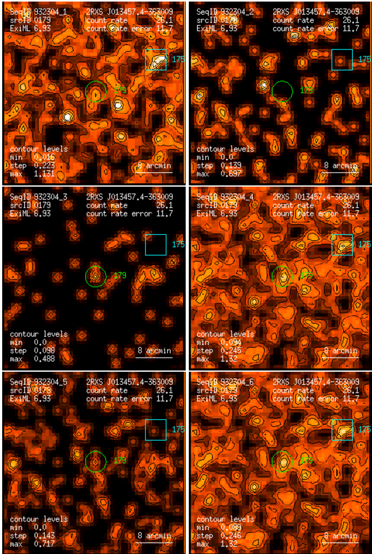
Figure 179: RASS 932304: detection 0179: band rate images, Gaussian filter: (1) PSPC channels 11 – 41, (2) 52 – 90, (3) 91 – 201, (4) 11 – 235, (5) 52 – 201, (6) 11 – 201. Broad band rates in counts/ks. Band rate contour levels in counts/ks/arcmin 2 .
