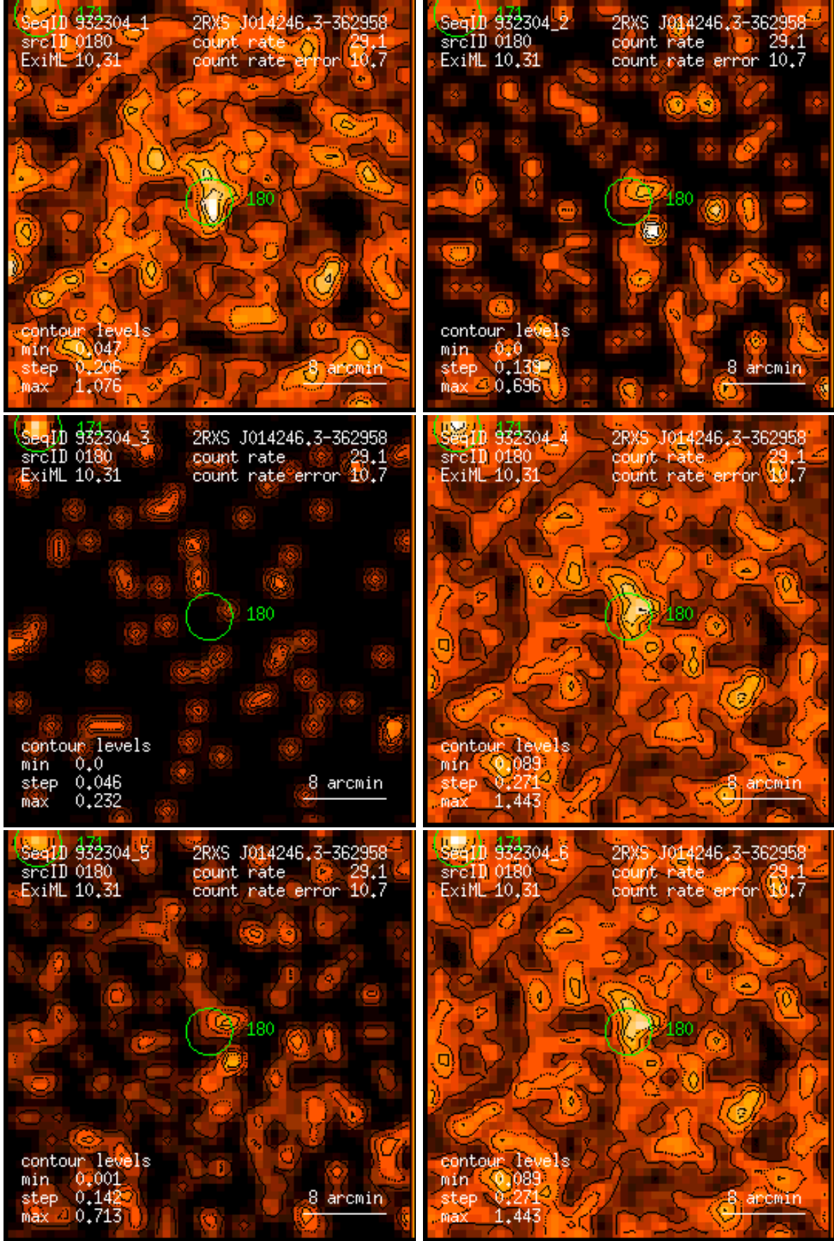
Figure 180: RASS 932304: detection 0180: band rate images, Gaussian filter: (1) PSPC channels 11 – 41, (2) 52 – 90, (3) 91 – 201, (4) 11 – 235, (5) 52 – 201, (6) 11 – 201. Broad band rates in counts/ks. Band rate contour levels in counts/ks/arcmin 2 .
