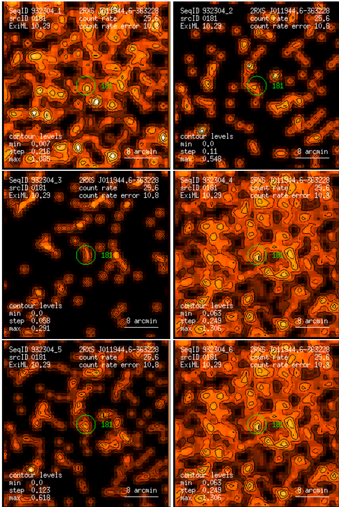
Figure 181: RASS 932304: detection 0181: band rate images, Gaussian filter: (1) PSPC channels 11 – 41, (2) 52 – 90, (3) 91 – 201, (4) 11 – 235, (5) 52 – 201, (6) 11 – 201. Broad band rates in counts/ks. Band rate contour levels in counts/ks/arcmin 2 .
