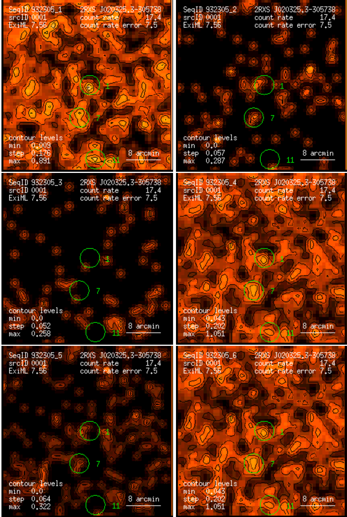
Figure 1: RASS 932305: detection 0001: band rate images, Gaussian filter: (1) PSPC channels 11 – 41, (2) 52 – 90, (3) 91 – 201, (4) 11 – 235, (5) 52 – 201, (6) 11 – 201. Broad band rates in counts/ks. Band rate contour levels in counts/ks/arcmin 2 .
