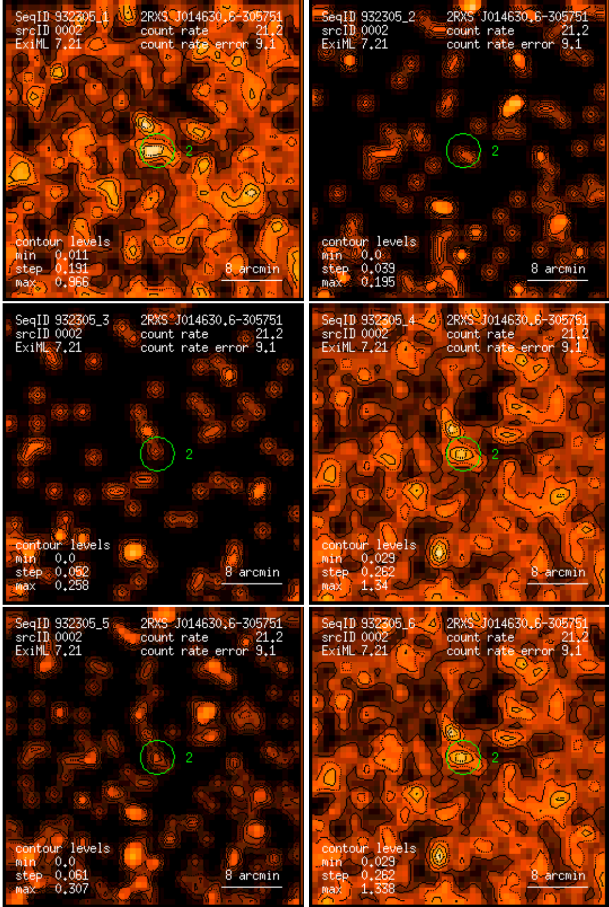
Figure 2: RASS 932305: detection 0002: band rate images, Gaussian filter: (1) PSPC channels 11 – 41, (2) 52 – 90, (3) 91 – 201, (4) 11 – 235, (5) 52 – 201, (6) 11 – 201. Broad band rates in counts/ks. Band rate contour levels in counts/ks/arcmin 2 .
