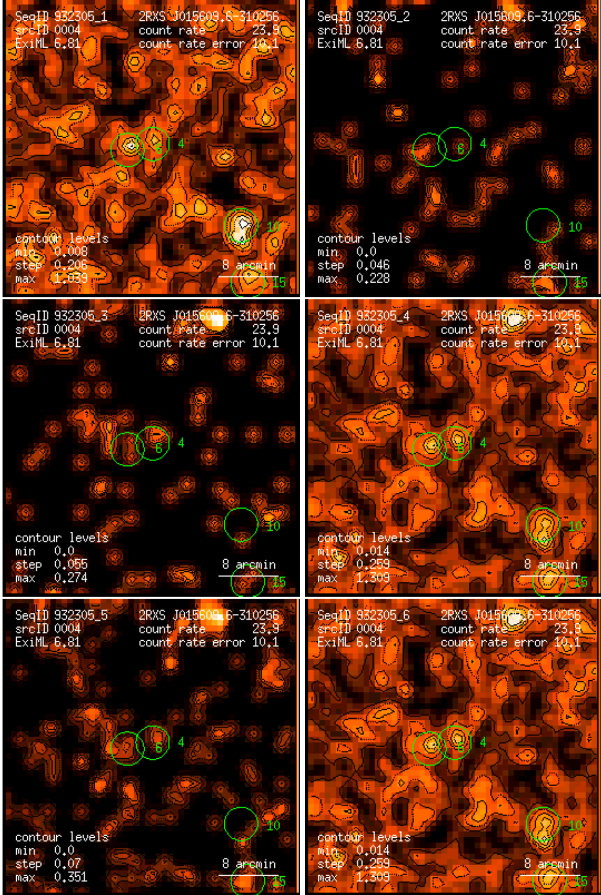
Figure 4: RASS 932305: detection 0004: band rate images, Gaussian filter: (1) PSPC channels 11 – 41, (2) 52 – 90, (3) 91 – 201, (4) 11 – 235, (5) 52 – 201, (6) 11 – 201. Broad band rates in counts/ks. Band rate contour levels in counts/ks/arcmin 2 .
