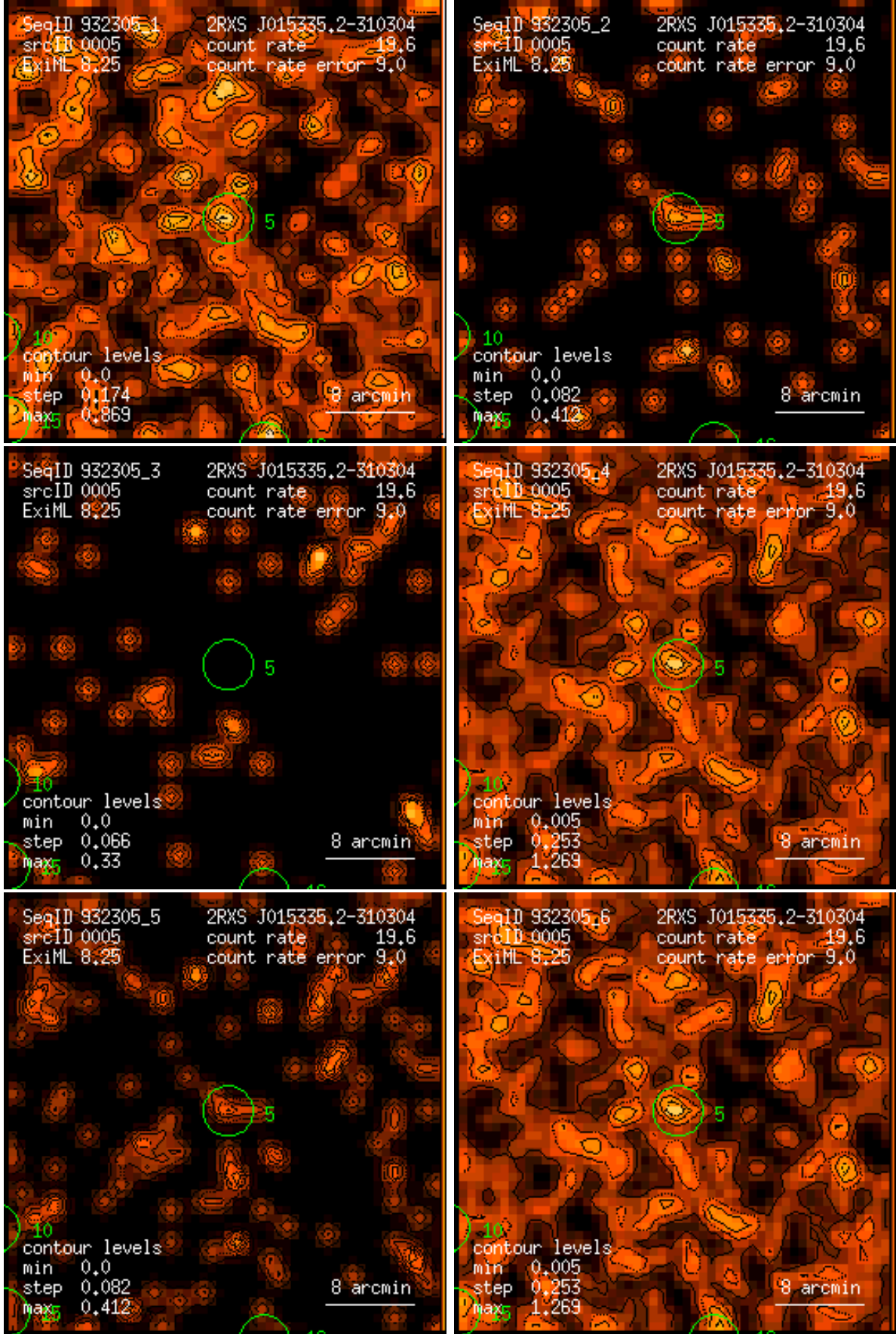
Figure 5: RASS 932305: detection 0005: band rate images, Gaussian filter: (1) PSPC channels 11 – 41, (2) 52 – 90, (3) 91 – 201, (4) 11 – 235, (5) 52 – 201, (6) 11 – 201. Broad band rates in counts/ks. Band rate contour levels in counts/ks/arcmin 2 .
