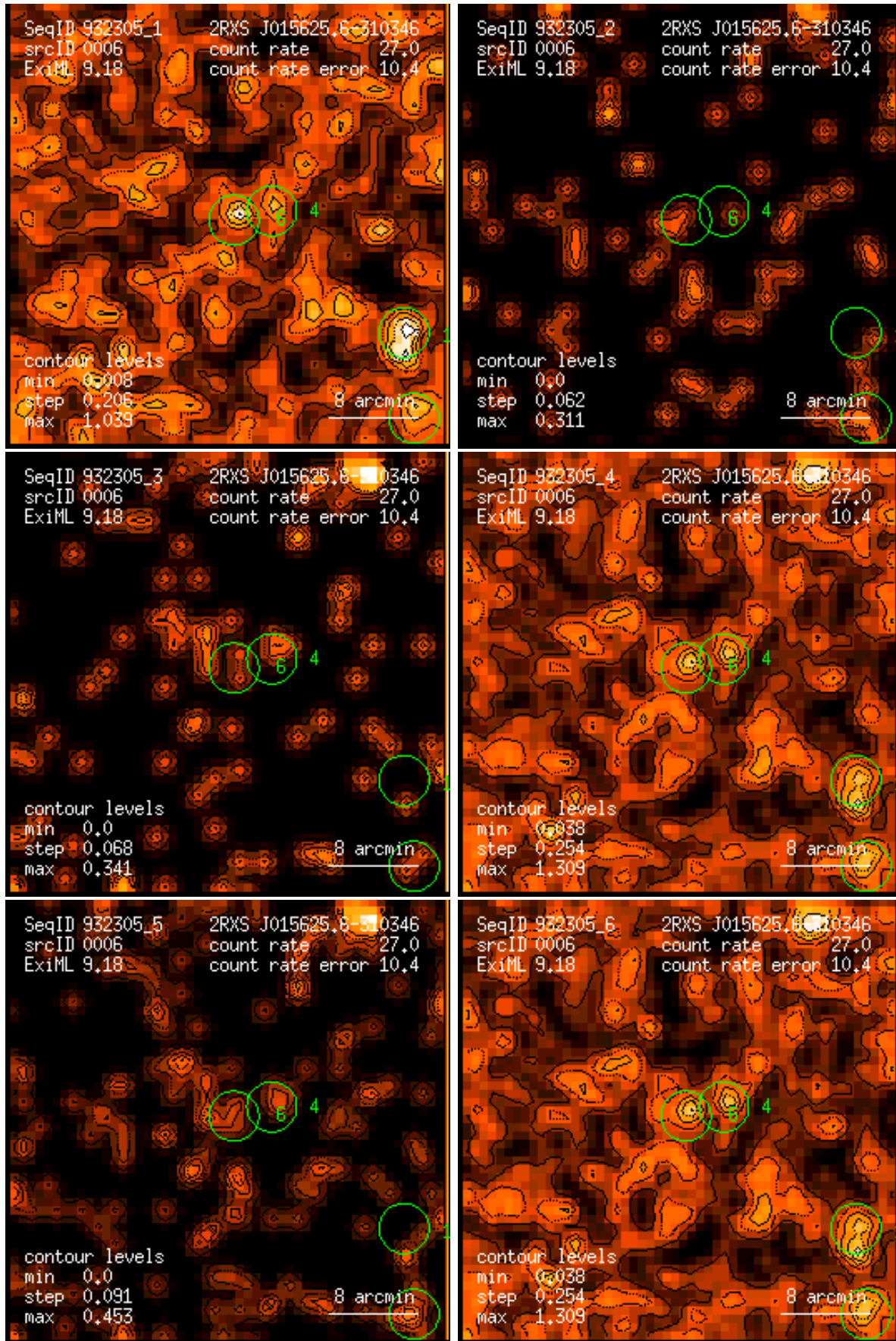
Figure 6: RASS 932305: detection 0006: band rate images, Gaussian filter: (1) PSPC channels 11 – 41, (2) 52 – 90, (3) 91 – 201, (4) 11 – 235, (5) 52 – 201, (6) 11 – 201. Broad band rates in counts/ks. Band rate contour levels in counts/ks/arcmin 2 .
