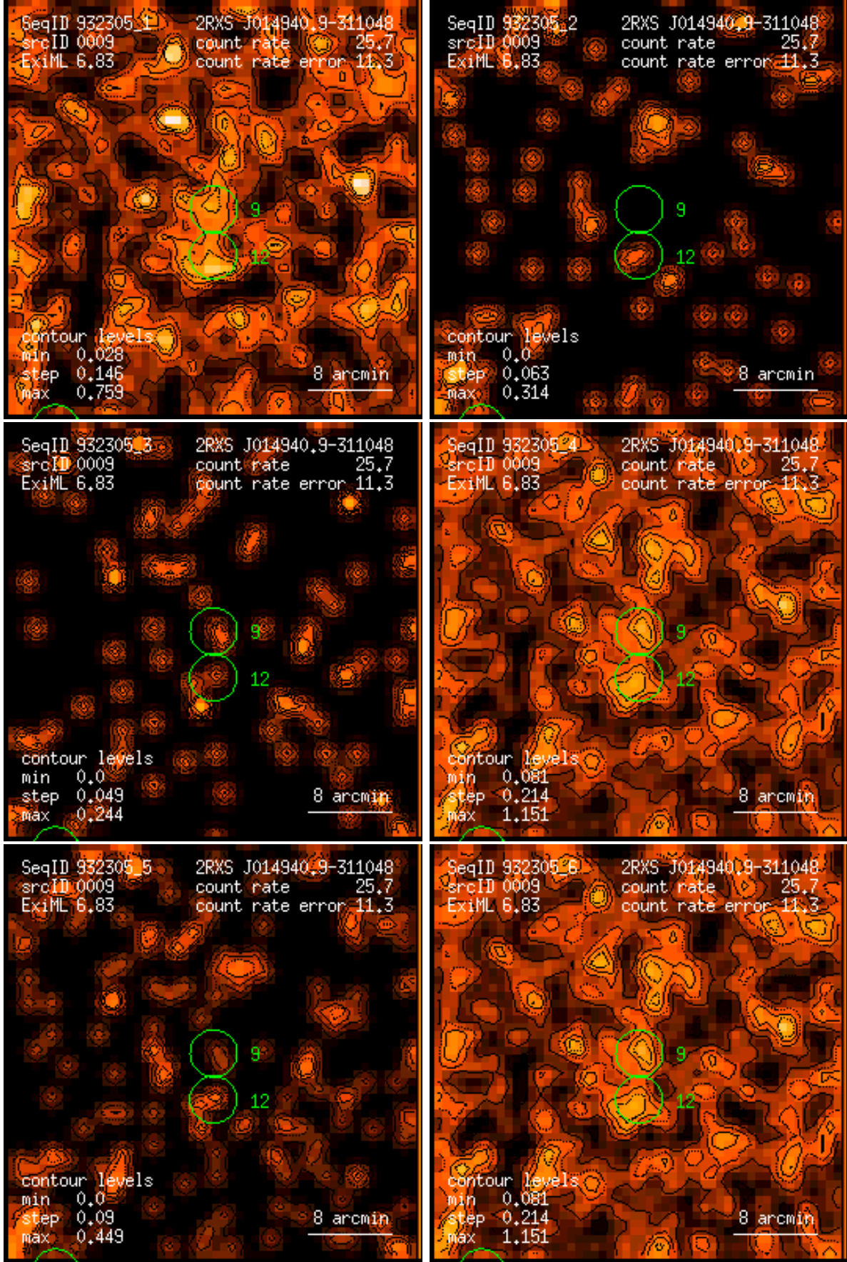
Figure 9: RASS 932305: detection 0009: band rate images, Gaussian filter: (1) PSPC channels 11 – 41, (2) 52 – 90, (3) 91 – 201, (4) 11 – 235, (5) 52 – 201, (6) 11 – 201. Broad band rates in counts/ks. Band rate contour levels in counts/ks/arcmin 2 .
