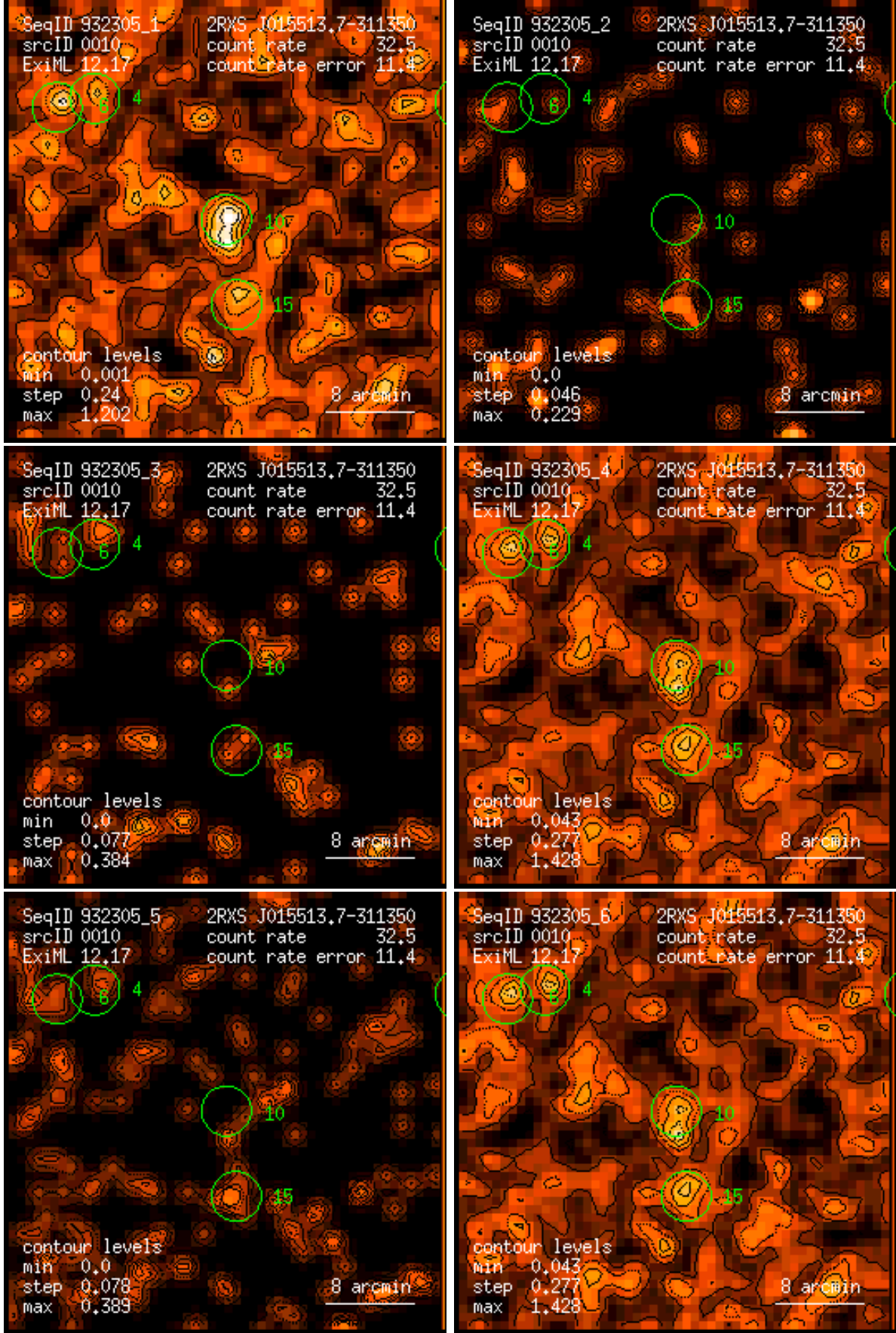
Figure 10: RASS 932305: detection 0010: band rate images, Gaussian filter: (1) PSPC channels 11 – 41, (2) 52 – 90, (3) 91 – 201, (4) 11 – 235, (5) 52 – 201, (6) 11 – 201. Broad band rates in counts/ks. Band rate contour levels in counts/ks/arcmin 2 .
