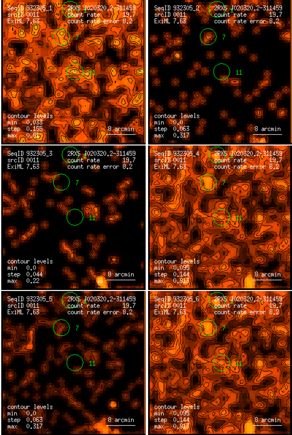
Figure 11: RASS 932305: detection 0011: band rate images, Gaussian filter: (1) PSPC channels 11 – 41, (2) 52 – 90, (3) 91 – 201, (4) 11 – 235, (5) 52 – 201, (6) 11 – 201. Broad band rates in counts/ks. Band rate contour levels in counts/ks/arcmin 2 .
