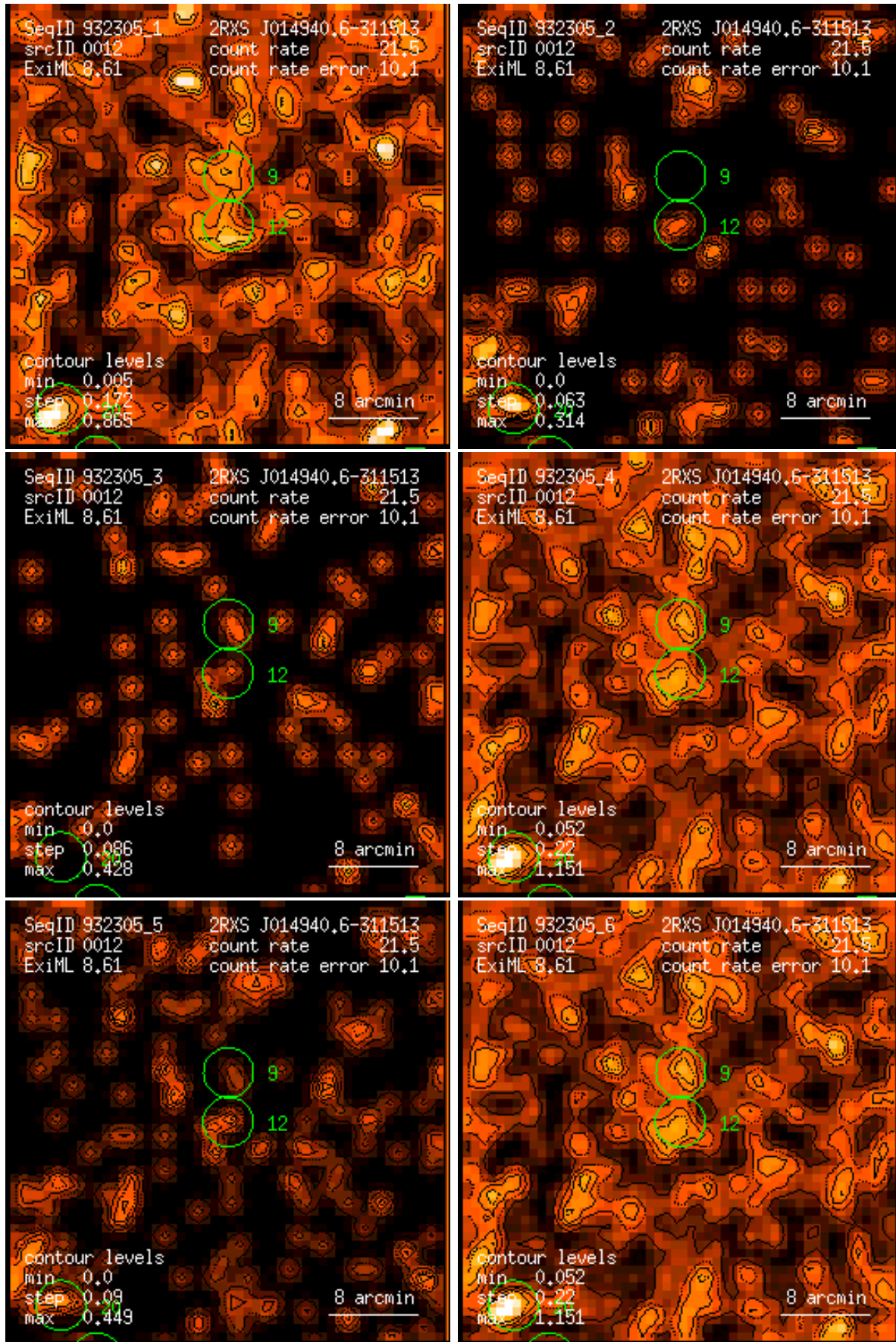
Figure 12: RASS 932305: detection 0012: band rate images, Gaussian filter: (1) PSPC channels 11 – 41, (2) 52 – 90, (3) 91 – 201, (4) 11 – 235, (5) 52 – 201, (6) 11 – 201. Broad band rates in counts/ks. Band rate contour levels in counts/ks/arcmin 2 .
