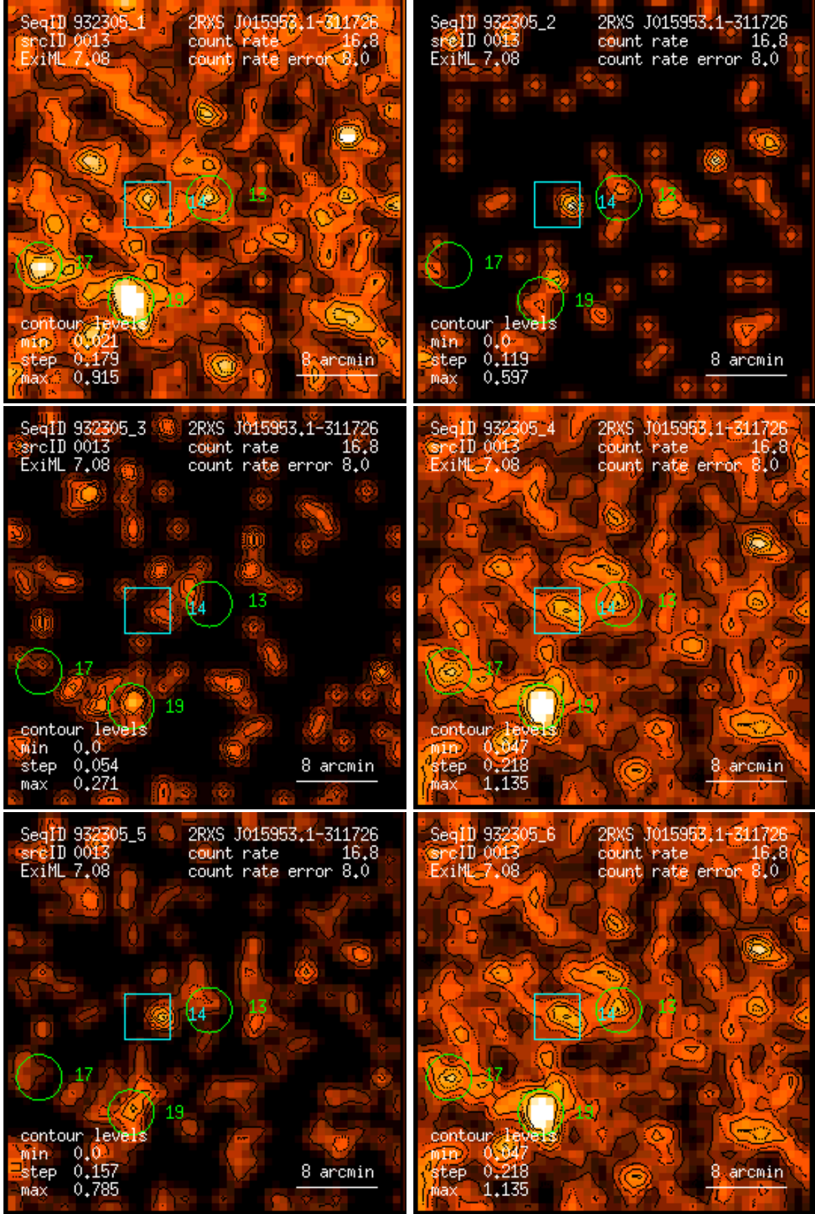
Figure 13: RASS 932305: detection 0013: band rate images, Gaussian filter: (1) PSPC channels 11 – 41, (2) 52 – 90, (3) 91 – 201, (4) 11 – 235, (5) 52 – 201, (6) 11 – 201. Broad band rates in counts/ks. Band rate contour levels in counts/ks/arcmin 2 .
