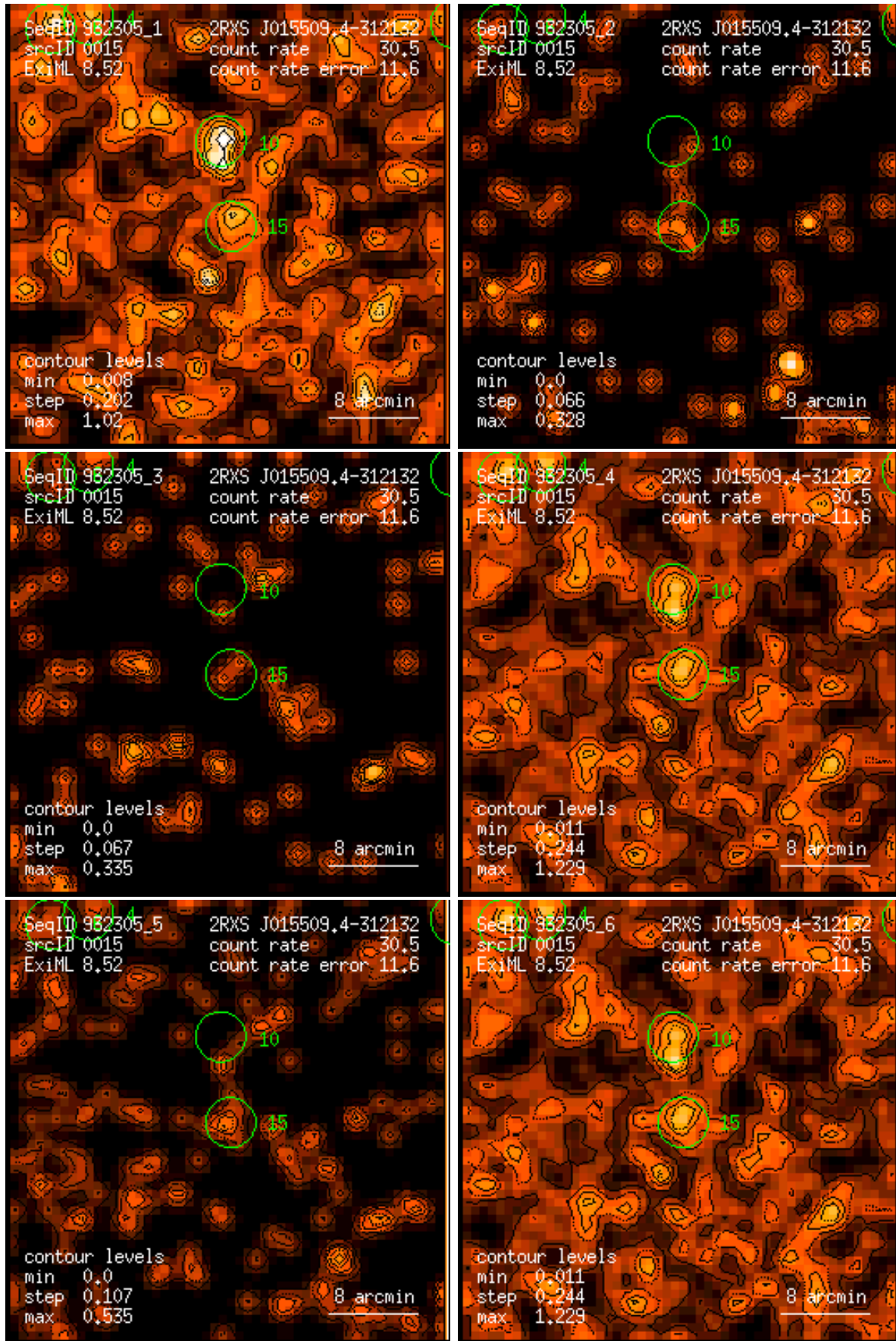
Figure 15: RASS 932305: detection 0015: band rate images, Gaussian filter: (1) PSPC channels 11 – 41, (2) 52 – 90, (3) 91 – 201, (4) 11 – 235, (5) 52 – 201, (6) 11 – 201. Broad band rates in counts/ks. Band rate contour levels in counts/ks/arcmin 2 .
