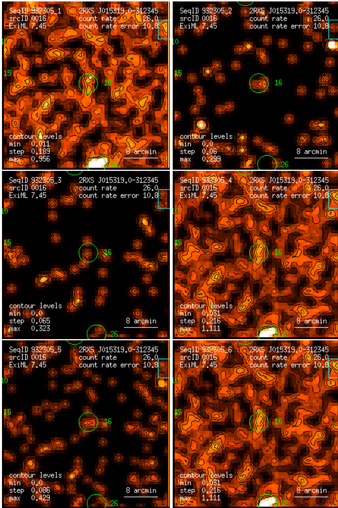
Figure 16: RASS 932305: detection 0016: band rate images, Gaussian filter: (1) PSPC channels 11 – 41, (2) 52 – 90, (3) 91 – 201, (4) 11 – 235, (5) 52 – 201, (6) 11 – 201. Broad band rates in counts/ks. Band rate contour levels in counts/ks/arcmin 2 .
