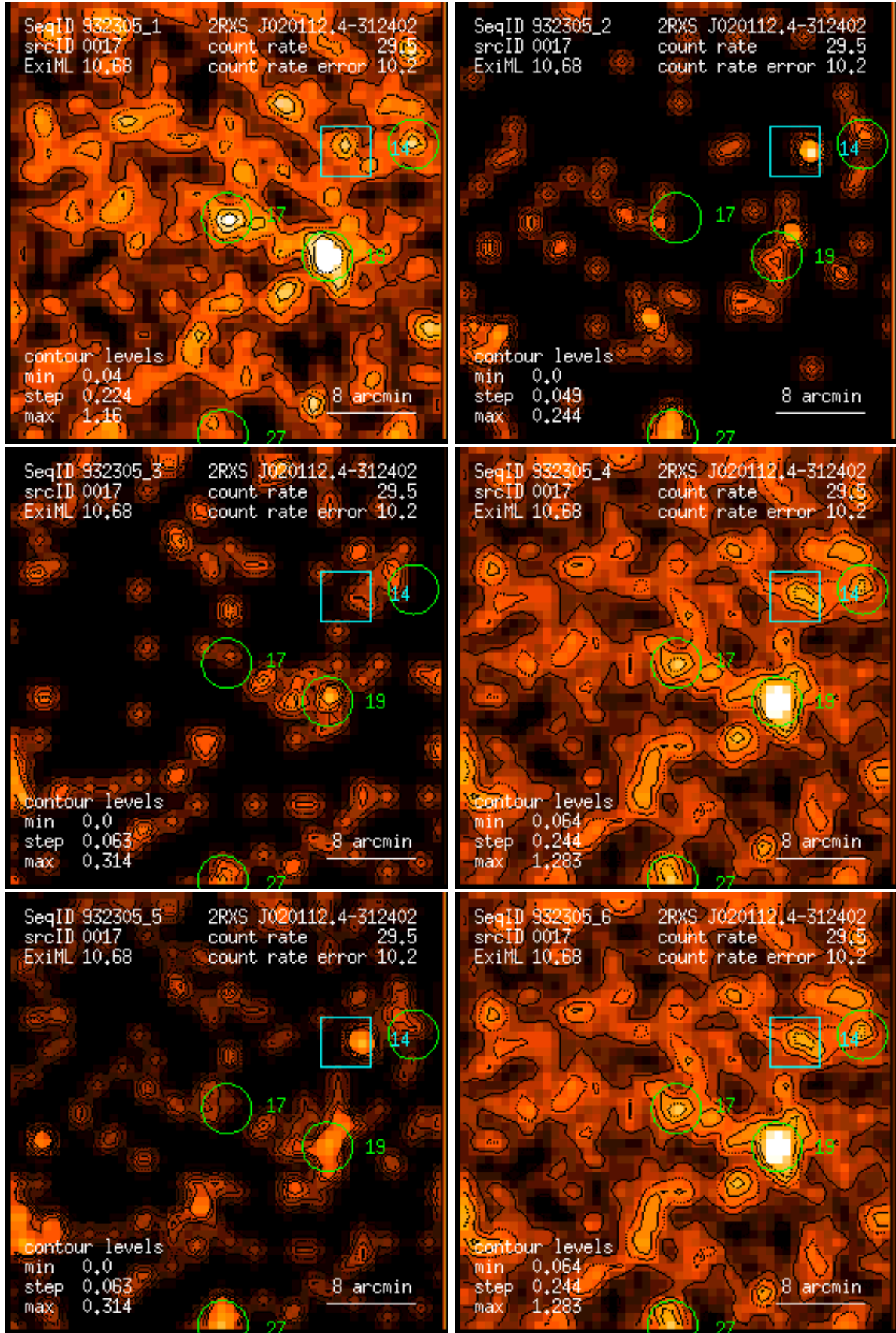
Figure 17: RASS 932305: detection 0017: band rate images, Gaussian filter: (1) PSPC channels 11 – 41, (2) 52 – 90, (3) 91 – 201, (4) 11 – 235, (5) 52 – 201, (6) 11 – 201. Broad band rates in counts/ks. Band rate contour levels in counts/ks/arcmin 2 .
