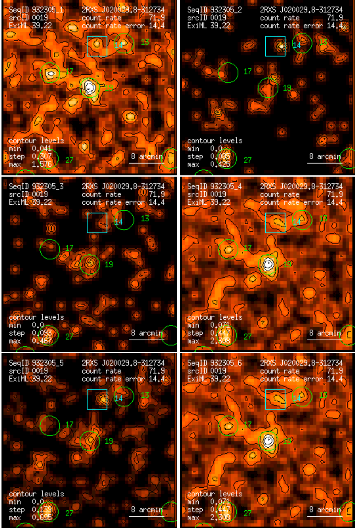
Figure 19: RASS 932305: detection 0019: band rate images, Gaussian filter: (1) PSPC channels 11 – 41, (2) 52 – 90, (3) 91 – 201, (4) 11 – 235, (5) 52 – 201, (6) 11 – 201. Broad band rates in counts/ks. Band rate contour levels in counts/ks/arcmin 2 .
