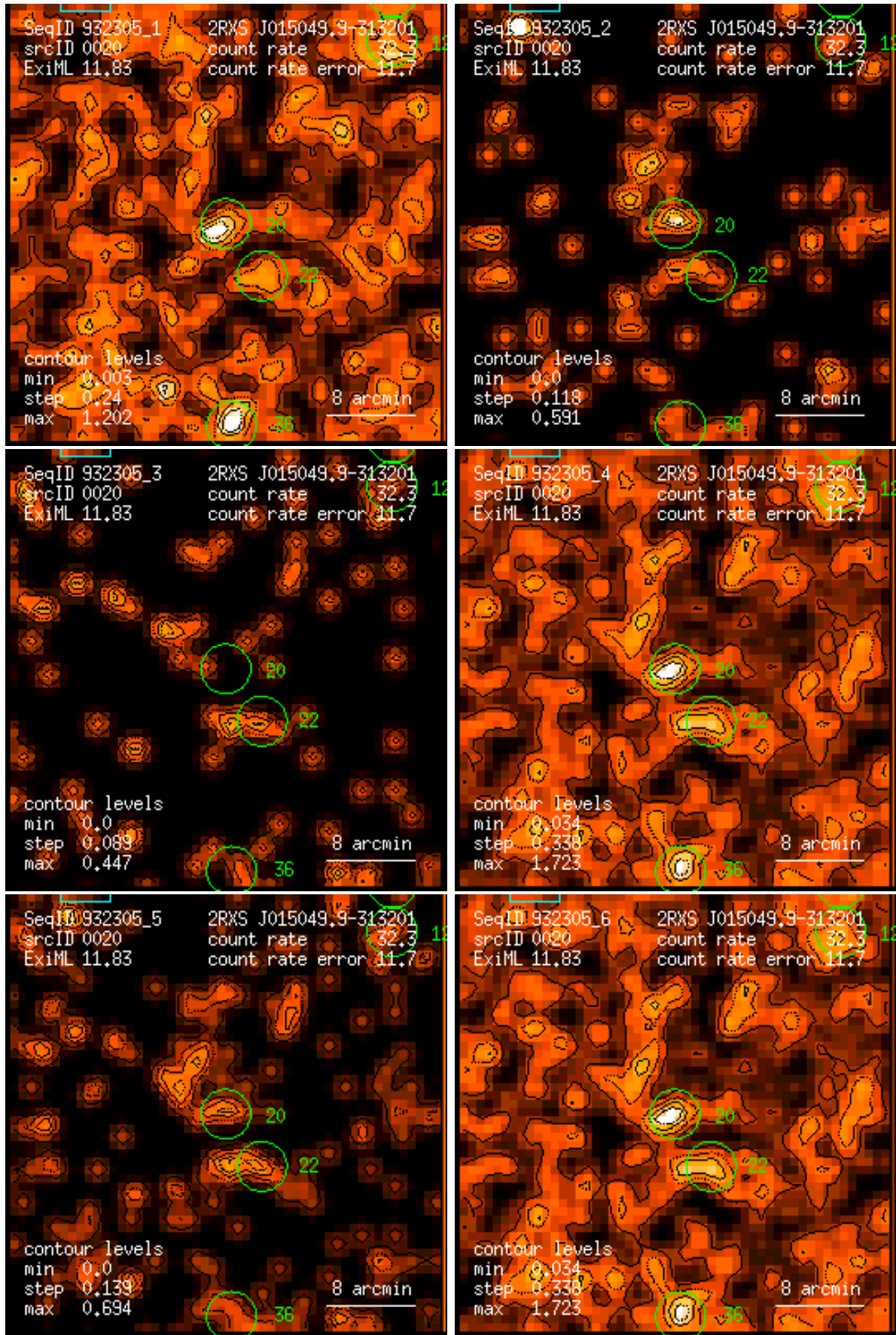
Figure 20: RASS 932305: detection 0020: band rate images, Gaussian filter: (1) PSPC channels 11 – 41, (2) 52 – 90, (3) 91 – 201, (4) 11 – 235, (5) 52 – 201, (6) 11 – 201. Broad band rates in counts/ks. Band rate contour levels in counts/ks/arcmin 2 .
