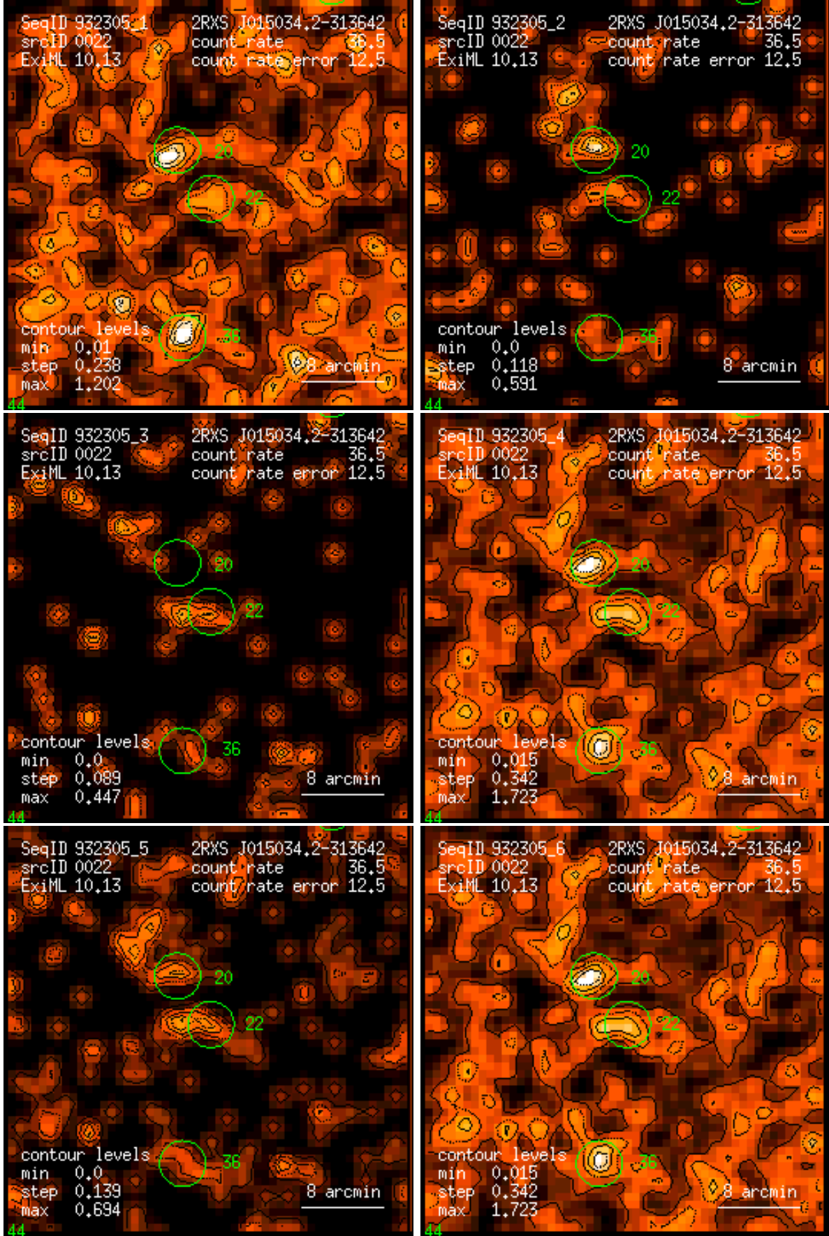
Figure 22: RASS 932305: detection 0022: band rate images, Gaussian filter: (1) PSPC channels 11 – 41, (2) 52 – 90, (3) 91 – 201, (4) 11 – 235, (5) 52 – 201, (6) 11 – 201. Broad band rates in counts/ks. Band rate contour levels in counts/ks/arcmin 2 .
