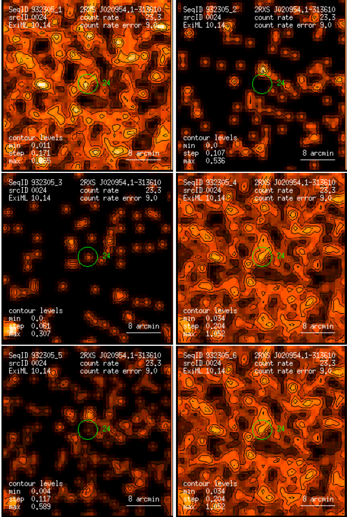
Figure 24: RASS 932305: detection 0024: band rate images, Gaussian filter: (1) PSPC channels 11 – 41, (2) 52 – 90, (3) 91 – 201, (4) 11 – 235, (5) 52 – 201, (6) 11 – 201. Broad band rates in counts/ks. Band rate contour levels in counts/ks/arcmin 2 .
