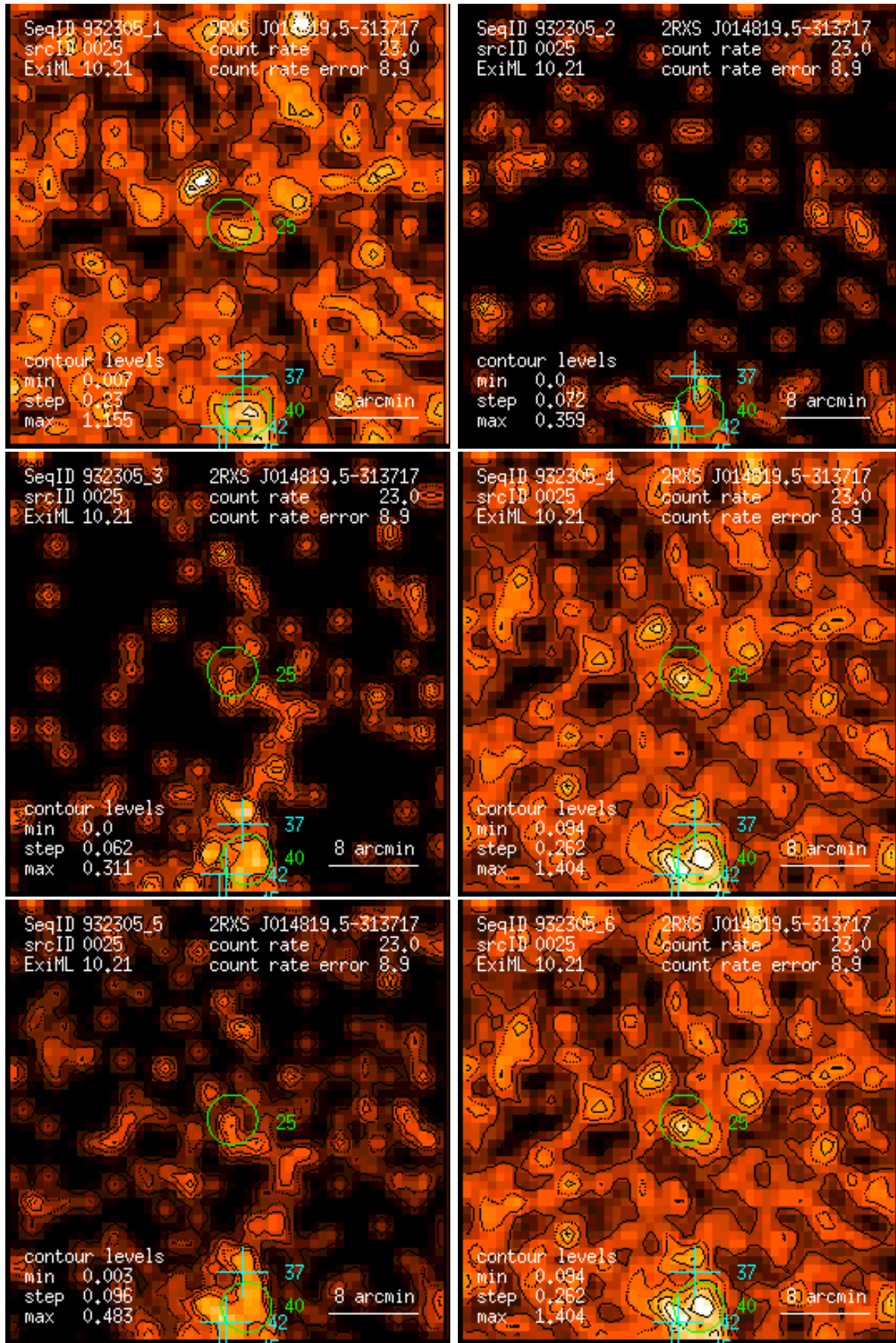
Figure 25: RASS 932305: detection 0025: band rate images, Gaussian filter: (1) PSPC channels 11 – 41, (2) 52 – 90, (3) 91 – 201, (4) 11 – 235, (5) 52 – 201, (6) 11 – 201. Broad band rates in counts/ks. Band rate contour levels in counts/ks/arcmin 2 .
