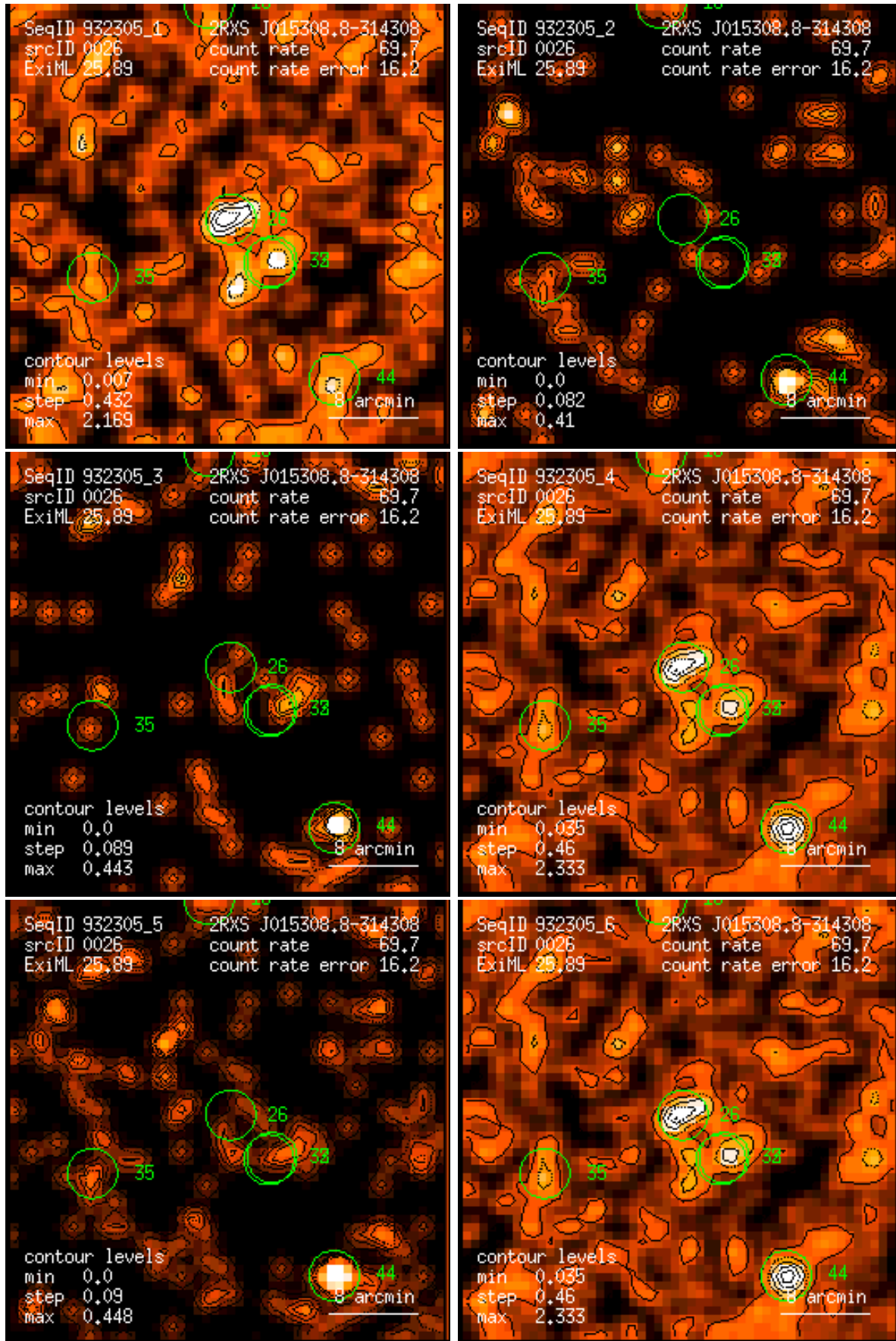
Figure 26: RASS 932305: detection 0026: band rate images, Gaussian filter: (1) PSPC channels 11 – 41, (2) 52 – 90, (3) 91 – 201, (4) 11 – 235, (5) 52 – 201, (6) 11 – 201. Broad band rates in counts/ks. Band rate contour levels in counts/ks/arcmin 2 .
