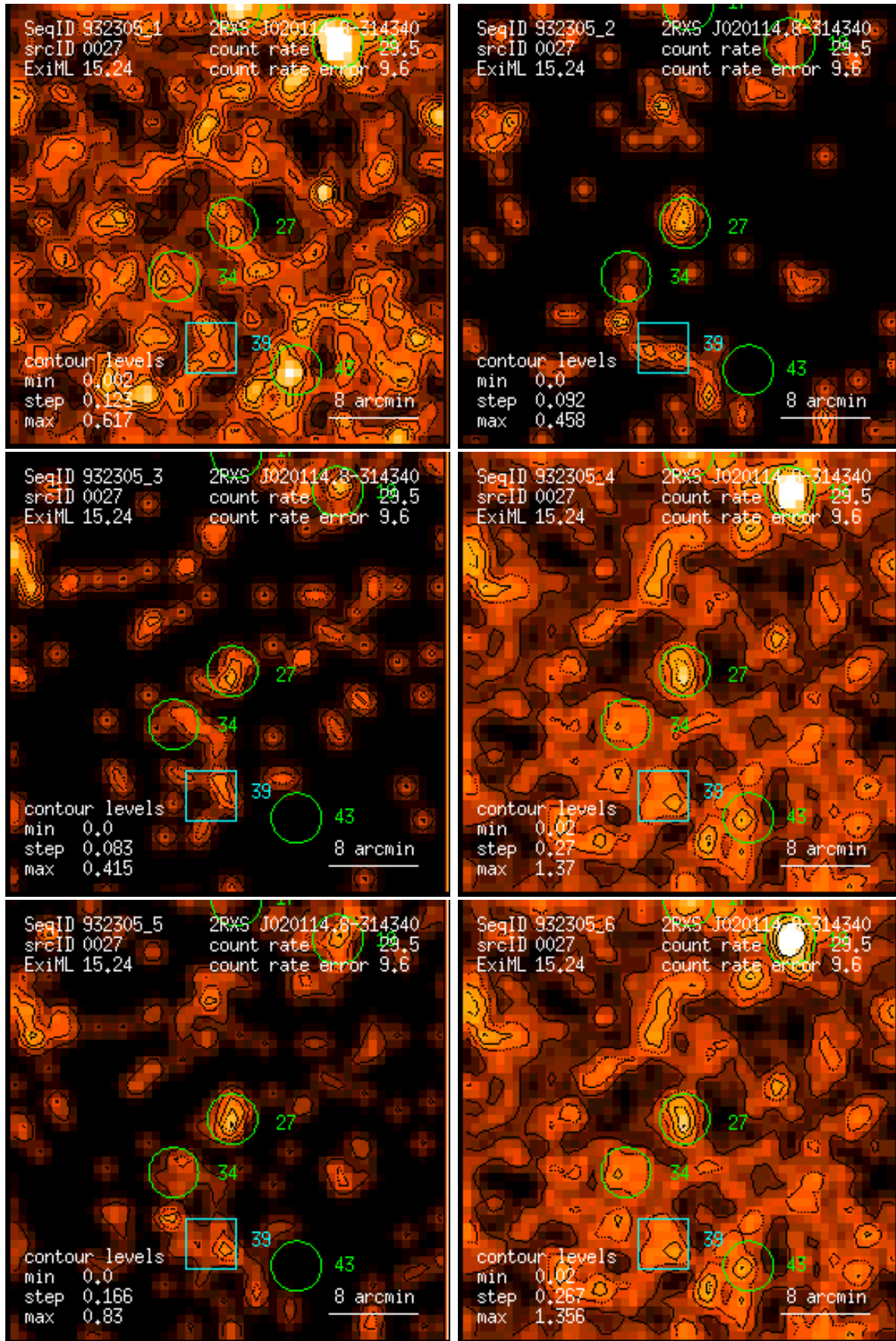
Figure 27: RASS 932305: detection 0027: band rate images, Gaussian filter: (1) PSPC channels 11 – 41, (2) 52 – 90, (3) 91 – 201, (4) 11 – 235, (5) 52 – 201, (6) 11 – 201. Broad band rates in counts/ks. Band rate contour levels in counts/ks/arcmin 2 .
