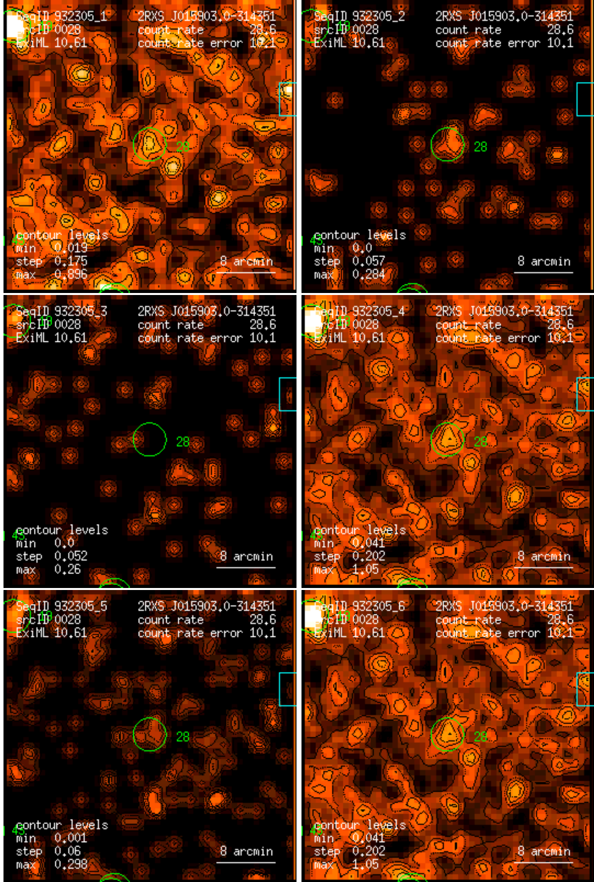
Figure 28: RASS 932305: detection 0028: band rate images, Gaussian filter: (1) PSPC channels 11 – 41, (2) 52 – 90, (3) 91 – 201, (4) 11 – 235, (5) 52 – 201, (6) 11 – 201. Broad band rates in counts/ks. Band rate contour levels in counts/ks/arcmin 2 .
